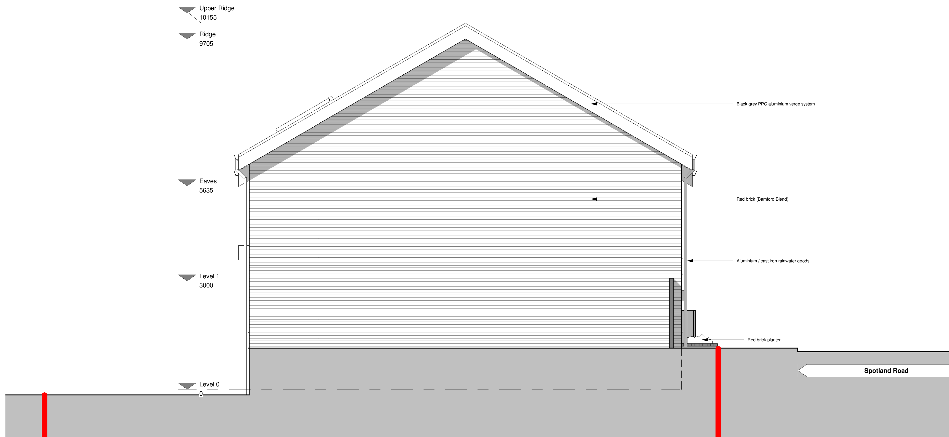
2 Proposed East Elevation 1 : 50
