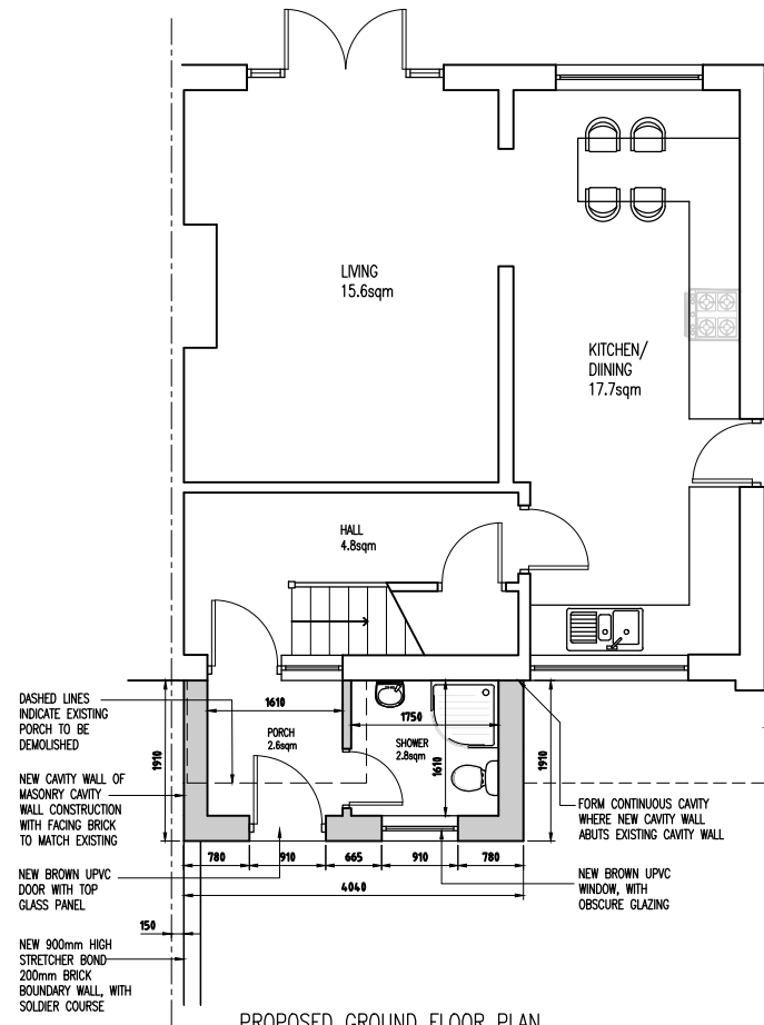
PROPOSED GROUND FLOOR PLAN 1:100 @ A3
