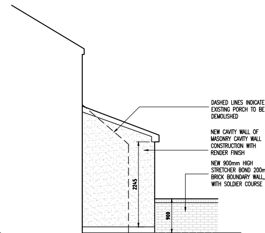
PROPOSED SIDE PORCH ELEVATION 1:100 @ A3
