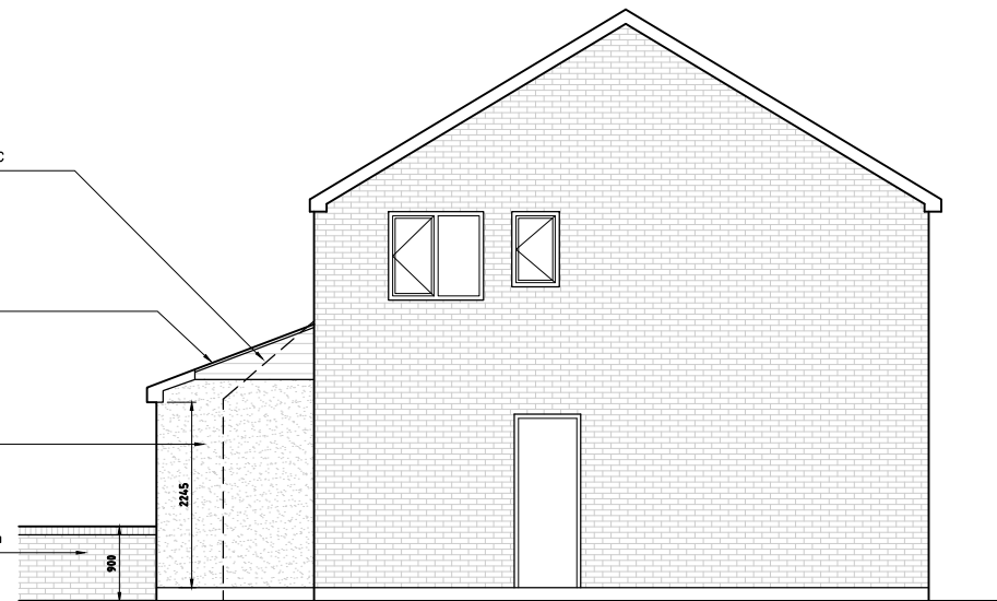
PROPOSED SIDE ELEVATION 1:100 @ A3
