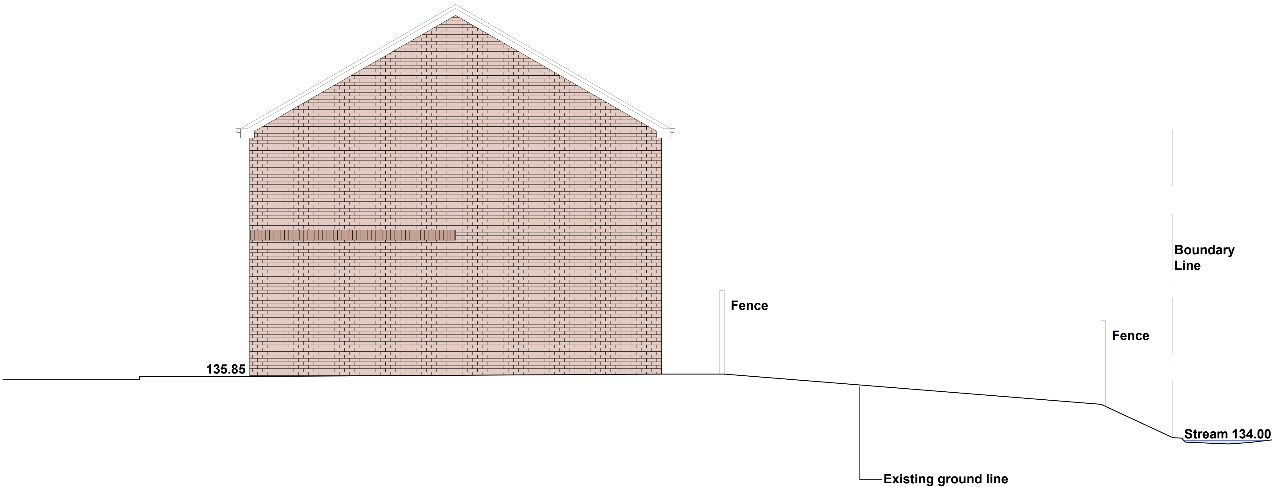
PROPOSED SITE SECTION Y - Y
