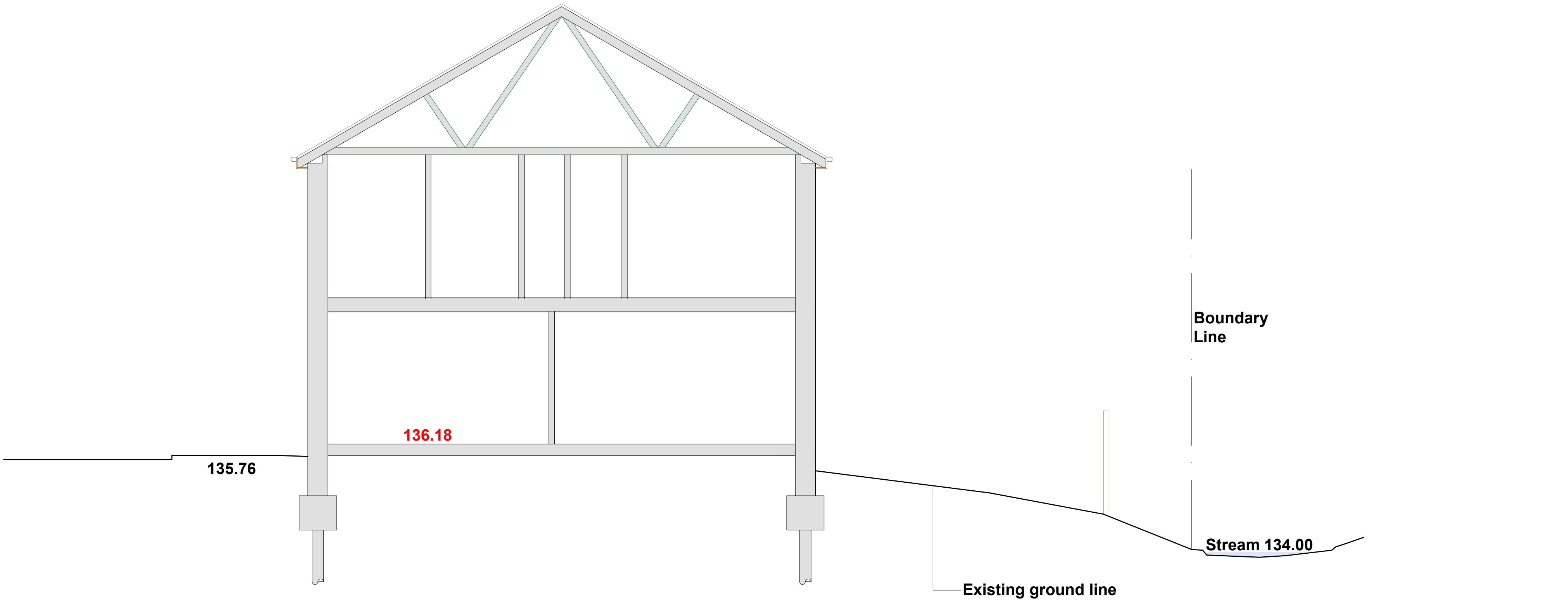
PROPOSED SITE SECTION X - X
