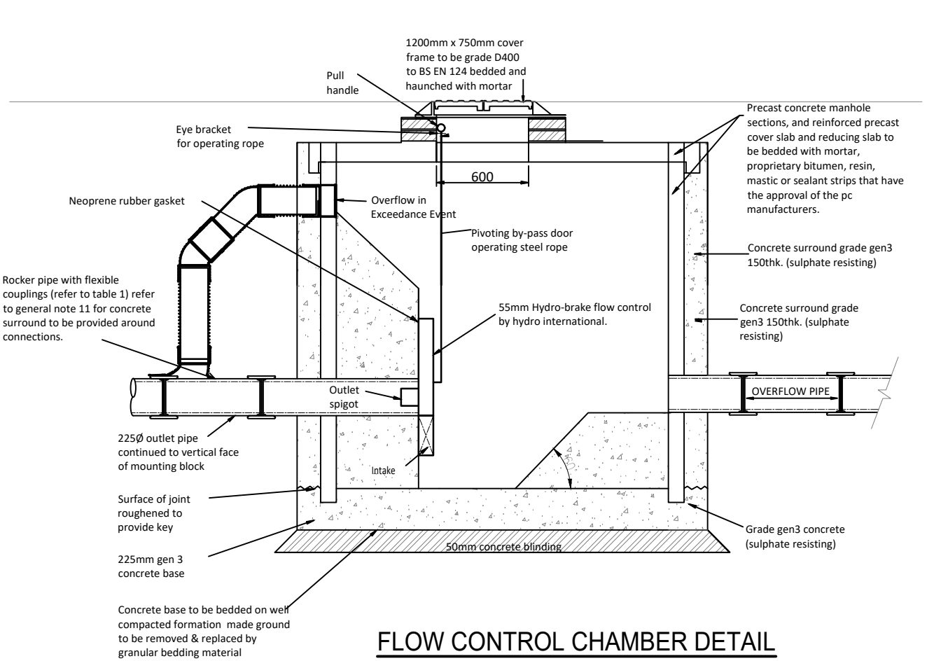
FLOW CONTROL CHAMBER DETAIL
