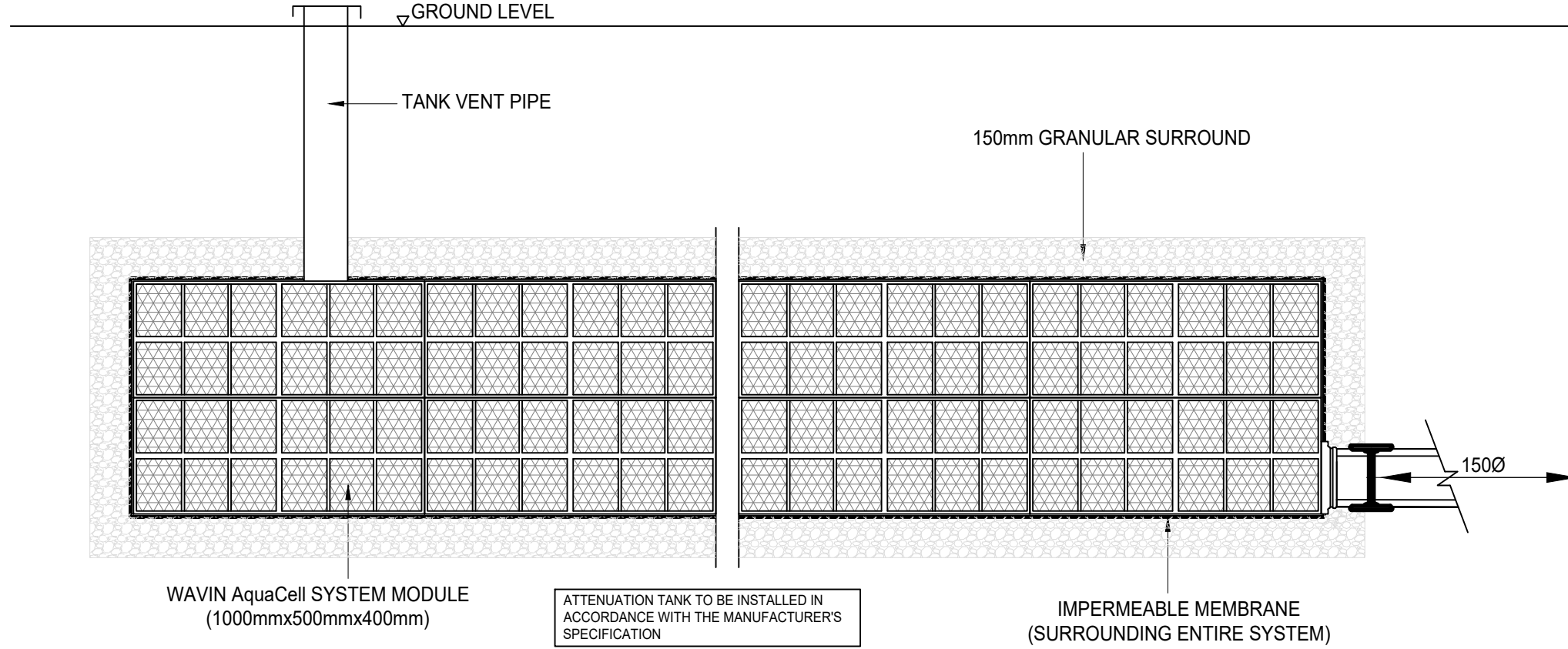
TYPICAL ATTENUATION TANK DETAIL
