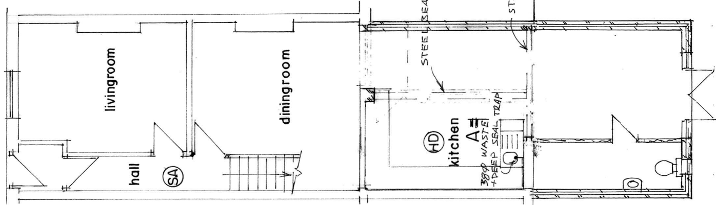
GROUND FLOOR PLAN (PROPOSED)
