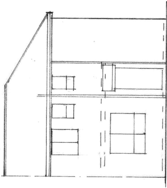
FRONT ELEVATION (EXISTING)
