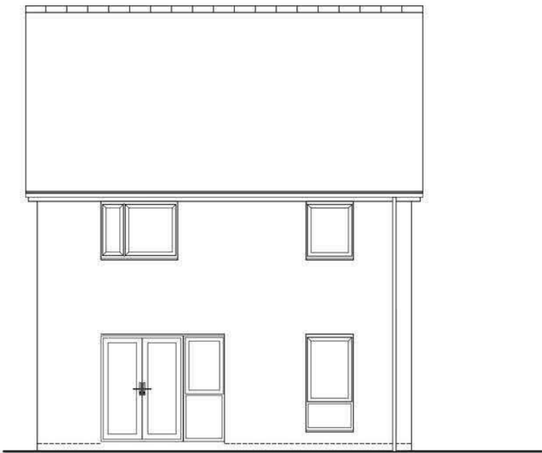
REAR ELEVATION DETACHED EMA43 (4B5P)
