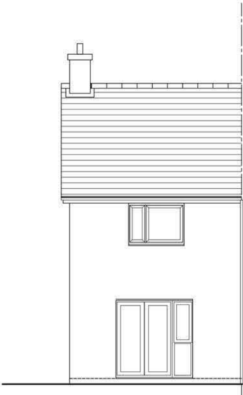
REAR ELEVATION END/SEMI DETACHED EMA22 (2B3P)
