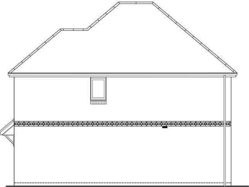
SIDE ELEVATION DETACHED
