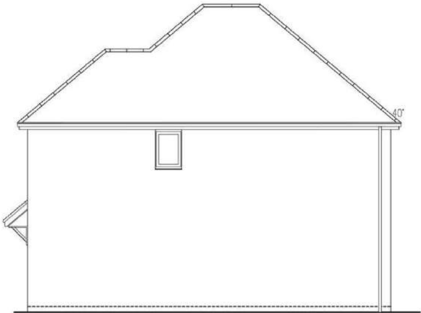
SIDE ELEVATION DETACHED EMG3 I (3B5P)
