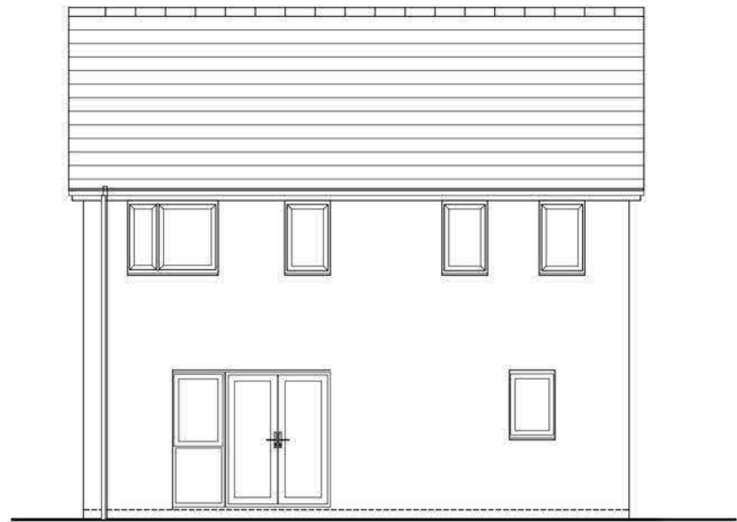
REAR ELEVATION DETACHED
