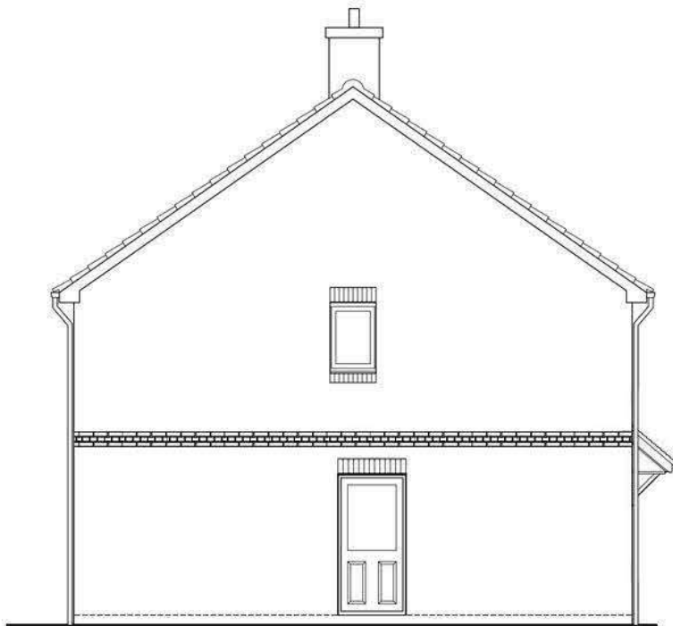
SIDE ELEVATION DETACHED EMA46 (4B7P)
