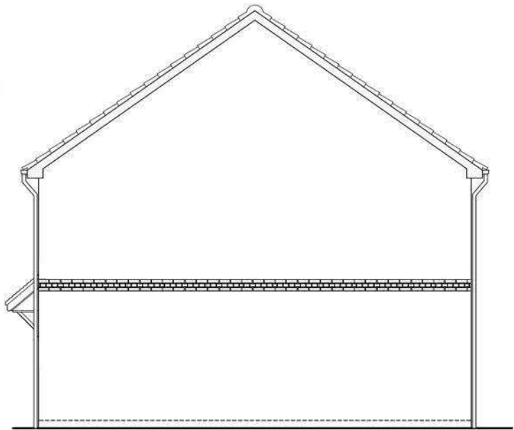
SIDE ELEVATION DETACHED EMA46 (4B7P)
