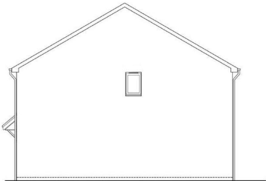
SIDE ELEVATION END/SEMI DETACHED EMA33 (2B4P)
