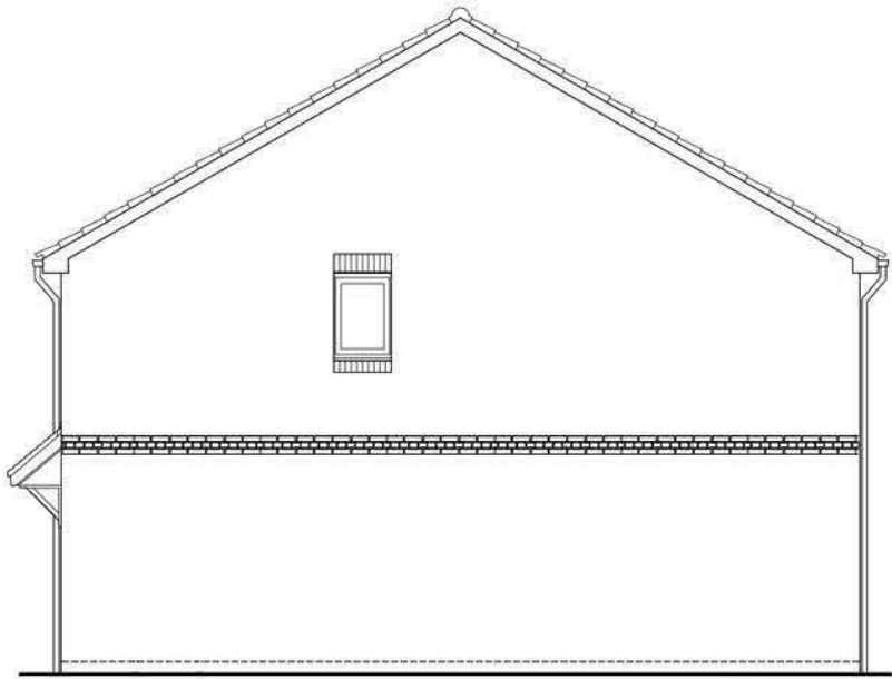
SIDE ELEVATION END/SEMI DETACHED EMA22 (2B3P)
