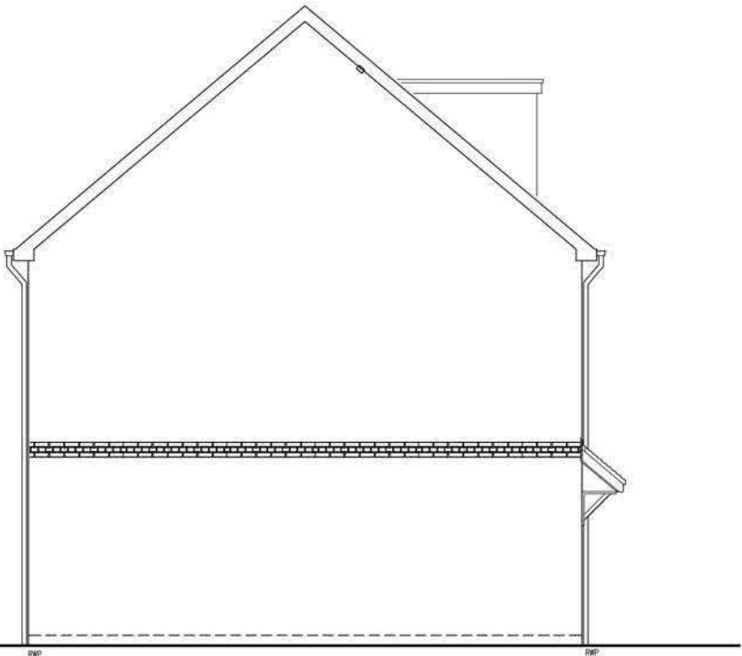
SIDE (LEFT) ELEVATION DETACHED
