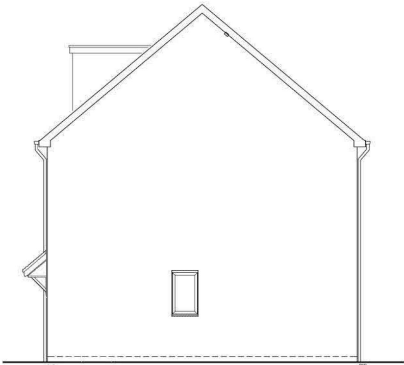
SIDE (RIGHT) ELEVATION DETACHED EMB5 I (5B7P)
