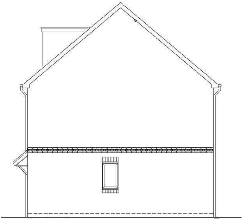
SIDE (RIGHT) ELEVATION DETACHED
