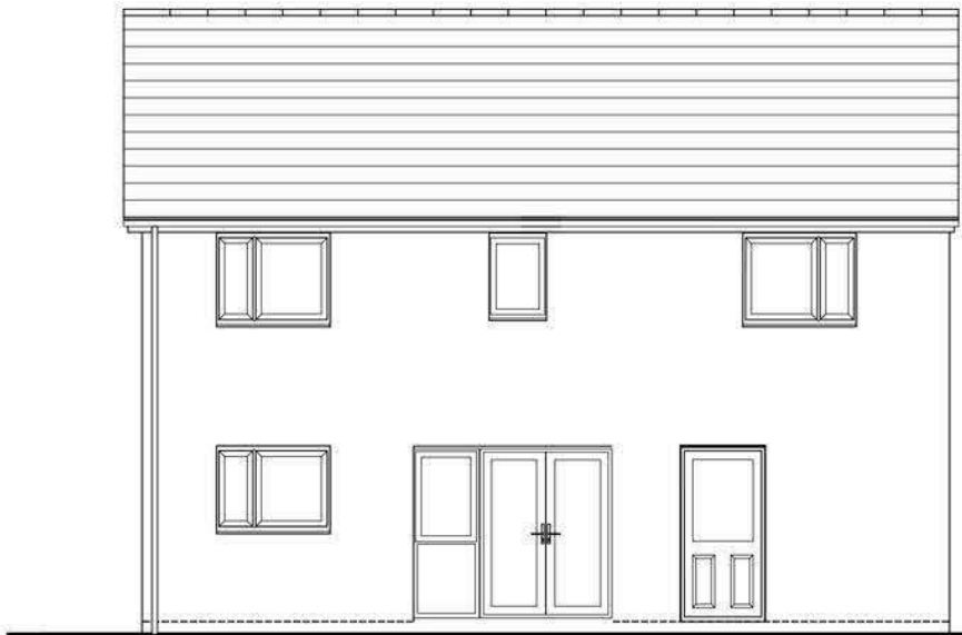
REAR ELEVATION DETACHED EMG43 (4B7P)
