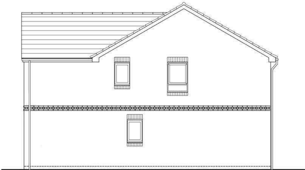
SIDE (RIGHT) ELEVATION DETACHED EMG43 (4B7P)
