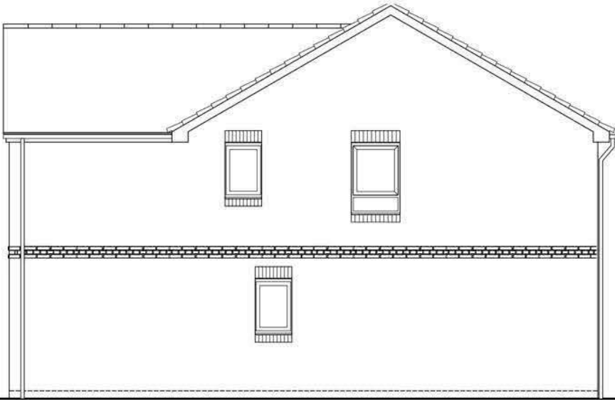
SIDE (RIGHT) ELEVATION DETACHED EMG43 (4B7P)
