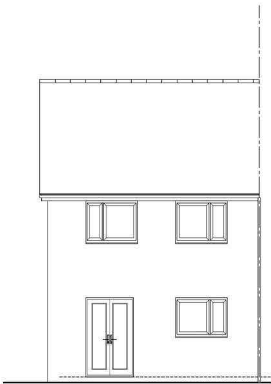
REAR ELEVATION END/SEMI DETACHED EMA33 (2B4P)
