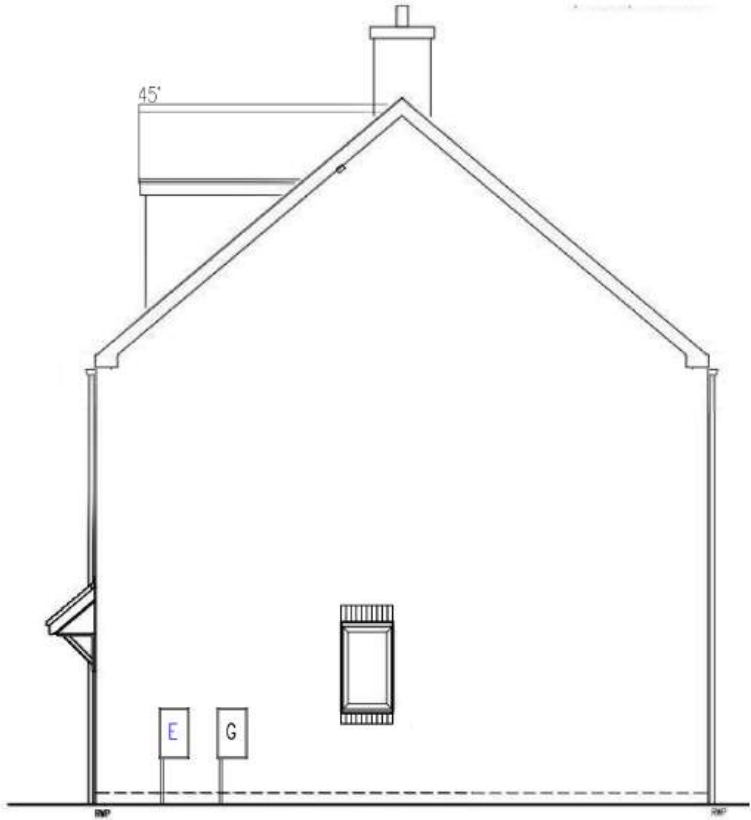
SIDE (RIGHT) ELEVATION DETACHED EMB5 I (5B7P)
