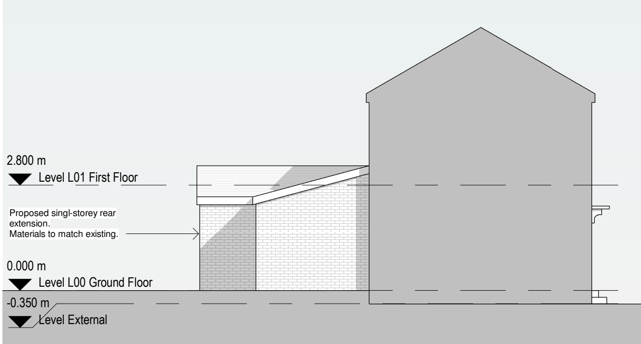
4 Proposed East Elevation 1 : 100
