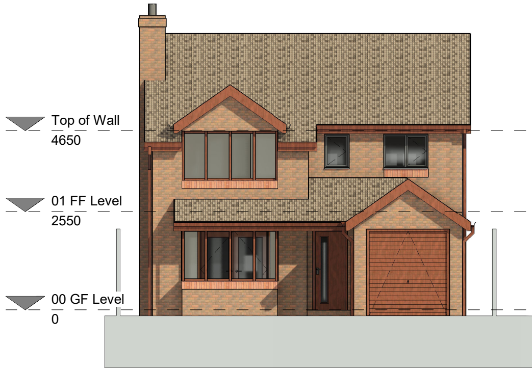
Front Elevation 1 : 100
