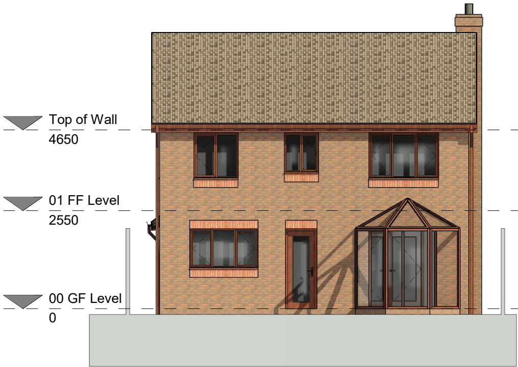
Rear Elevation 1 : 100
