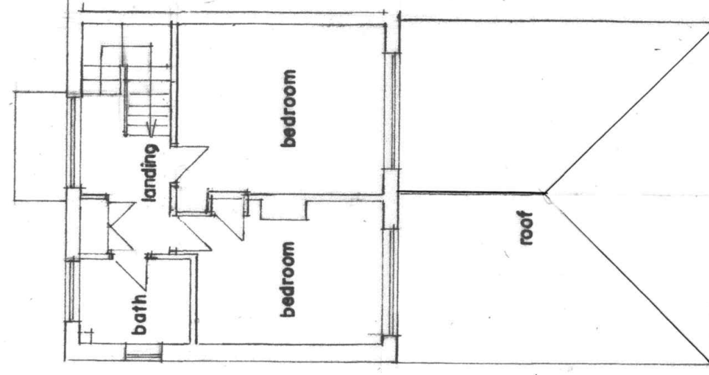
FIRST FLOOR PLAN (EXISTING)
