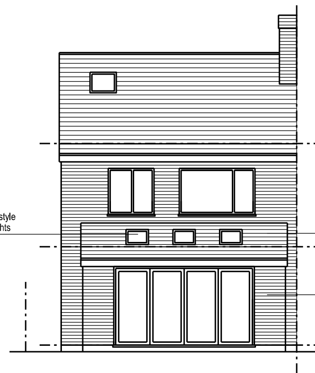
South Elevation
