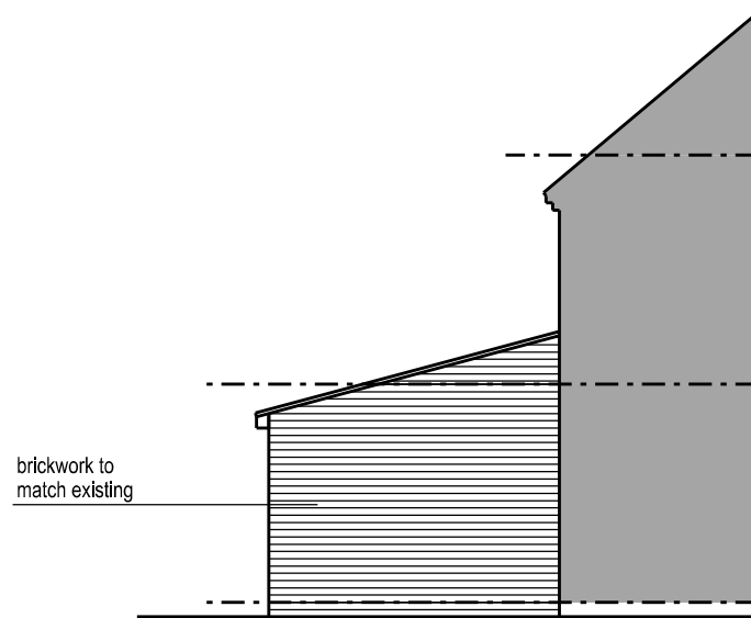
East Elevation
