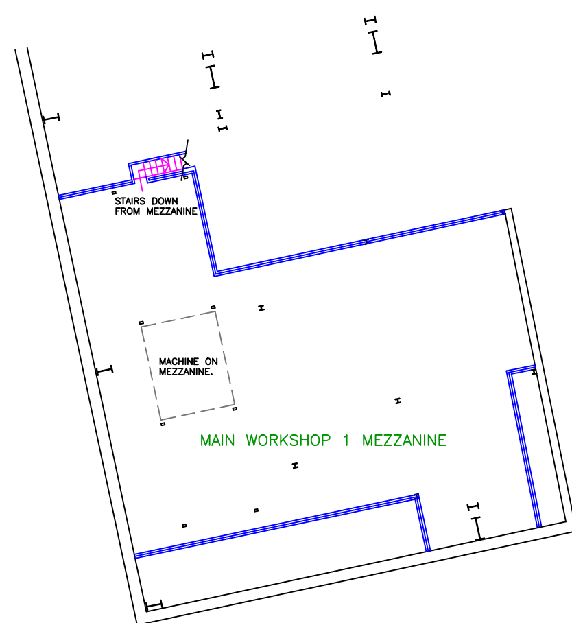
EXISTING FIRST FLOOR MAIN WORKSHOP 1 MEZZANINE PLAN
