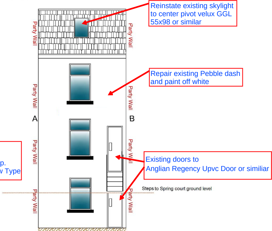
PROPOSED REAR ELEVATION 1:50 @ A1
