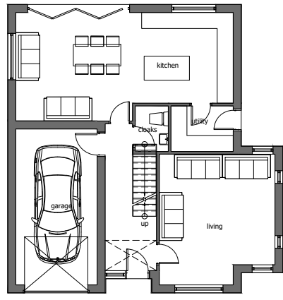
ground floor plan (orangery removed)
