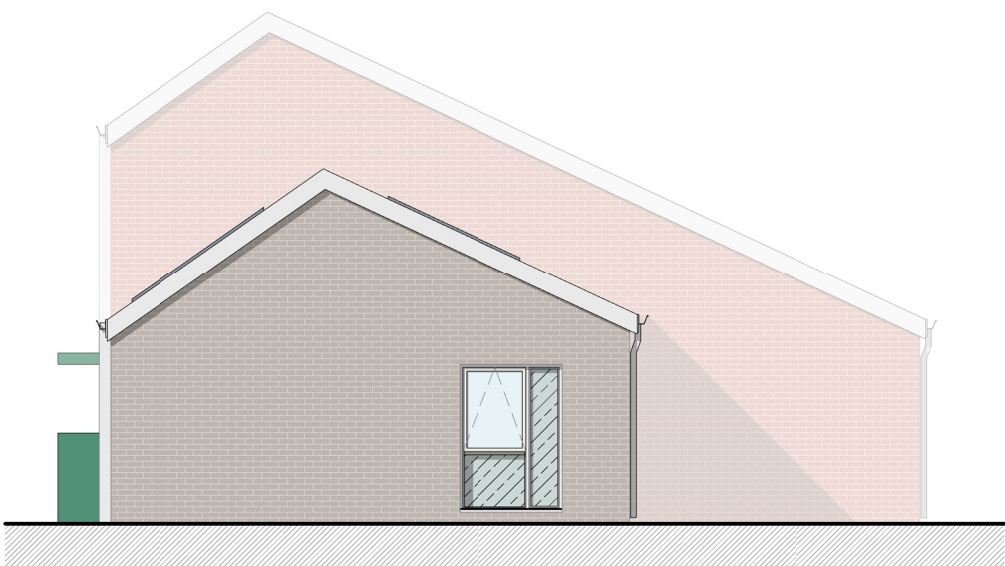
Side 2 Elevation 1:100
