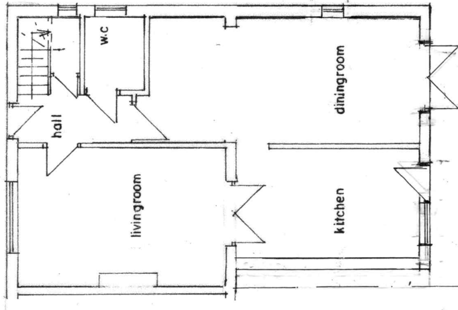
GROUND FLOOR PLAN (EXISTING)
