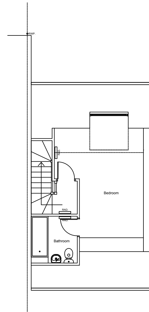
Existing Second Floor Plan (Loft)
