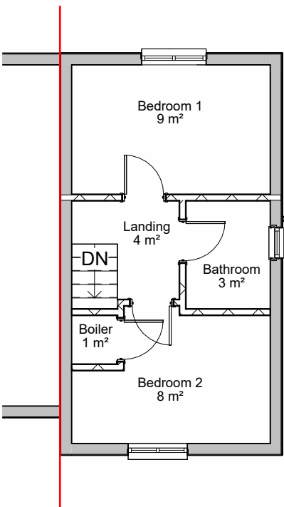
Ex First Floor 1 : 100
