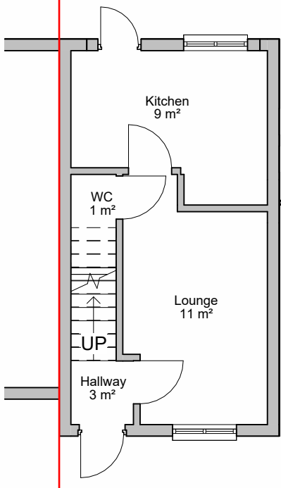
Ex Ground Floor 1 : 100
