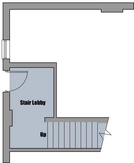
Part Ground Floor Plan
