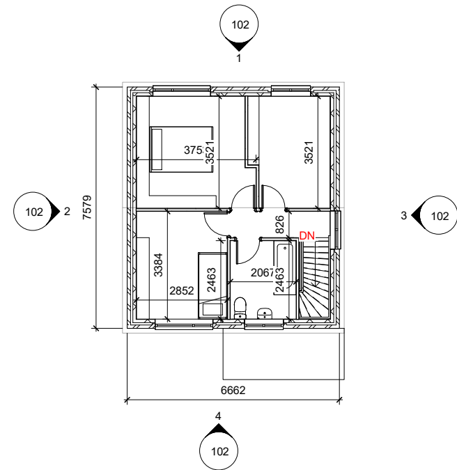
Existing First Floor Plan 1 : 100
