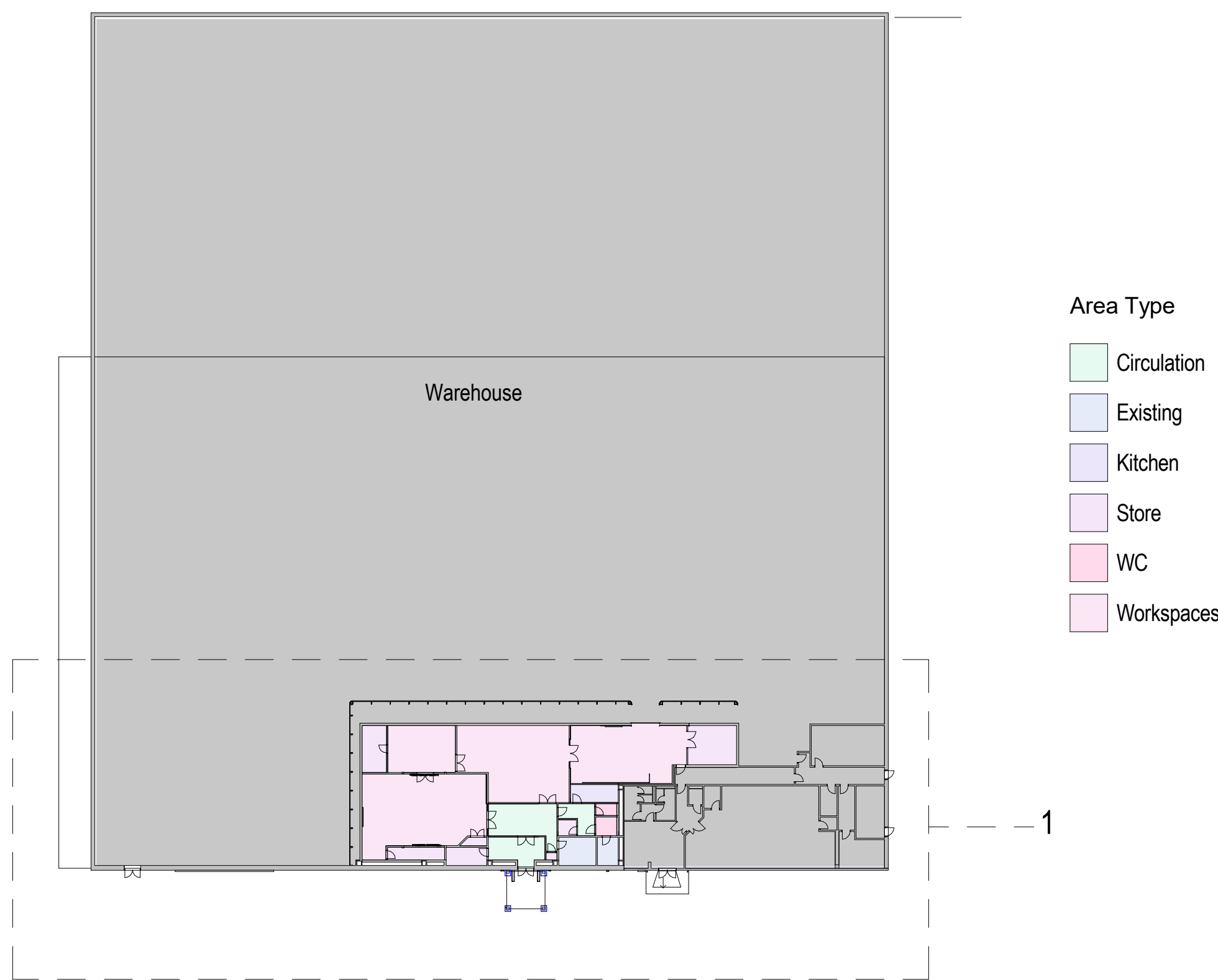
Level 0 (Ground Floor) Warehouse Proposed Plan
