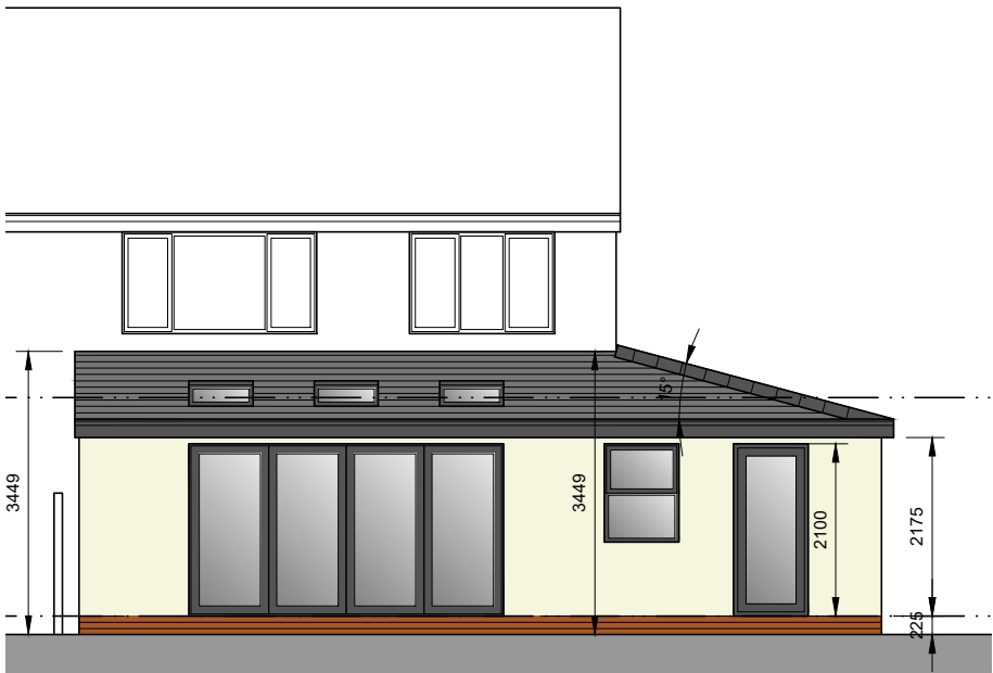
South Facing Rear Elevation
