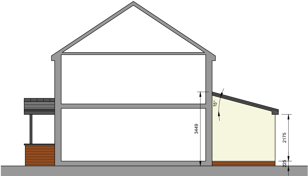
West Facing Side Elevational Section
