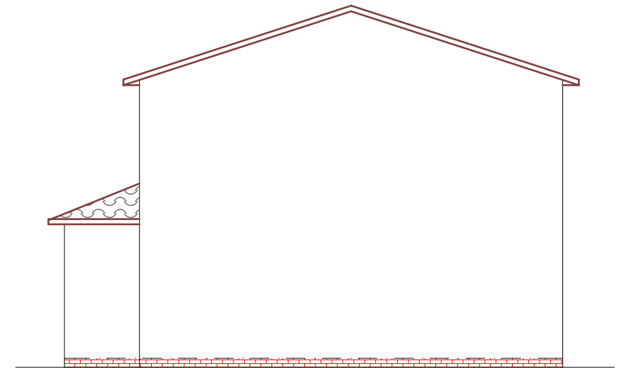
Side Elevation 1:100
