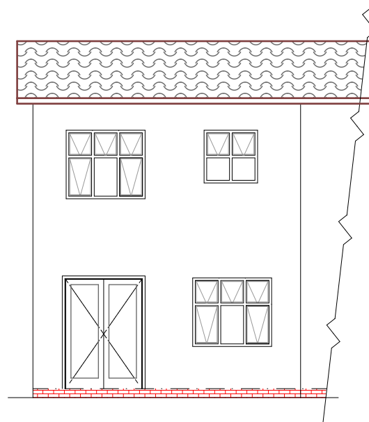
Rear Elevation 1:100
