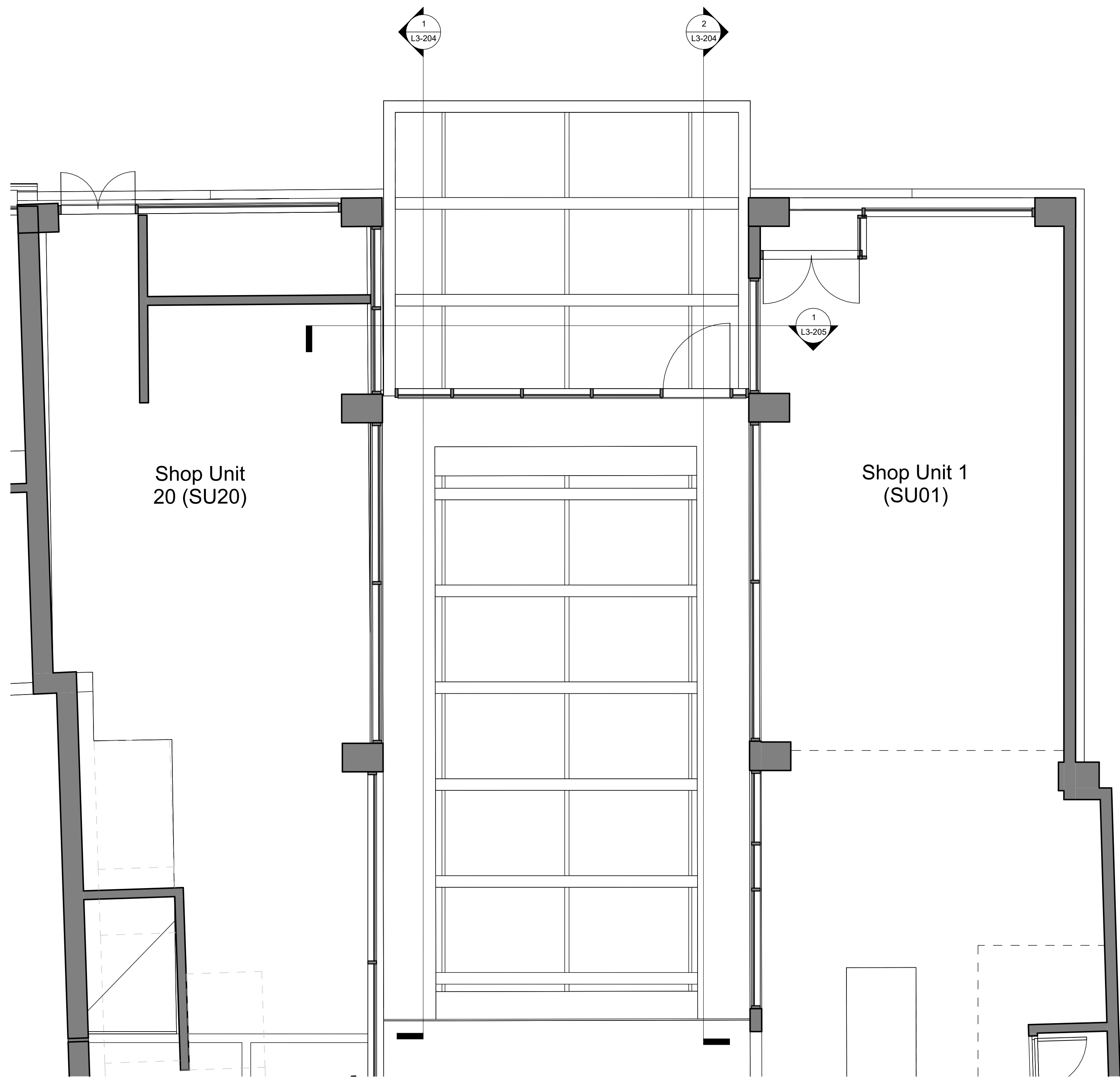
1 Entrance Lobby - Ceiling Plan (Existing) 1 : 50
