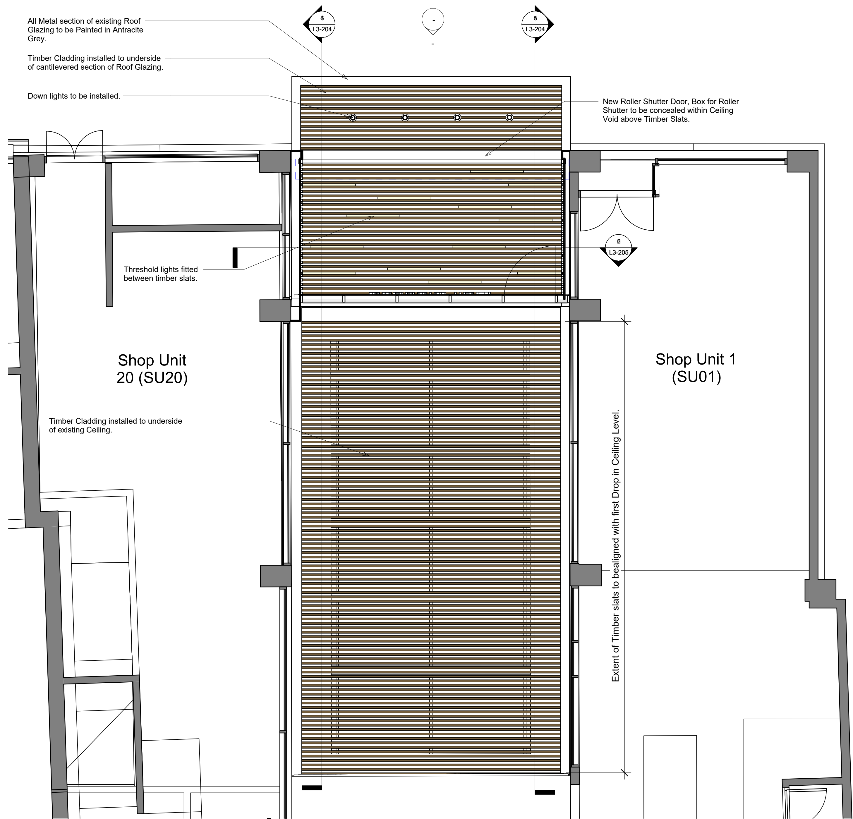
2 Entrance Lobby - Ceiling Plan (Proposed) 1 : 50
