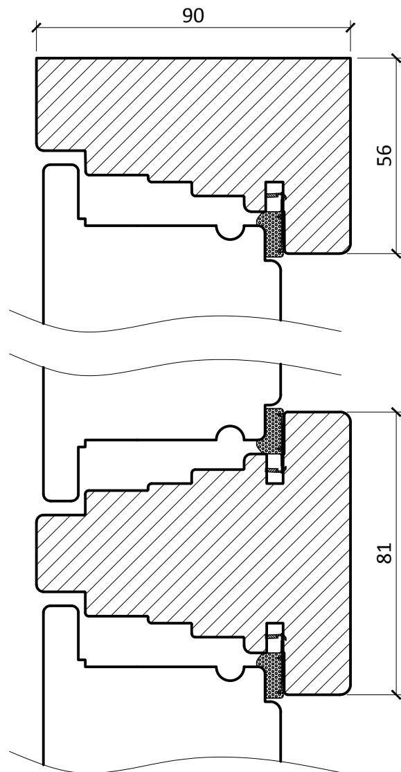
Square frame
