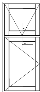
TOP HUNG OVER SIDE HUNG
