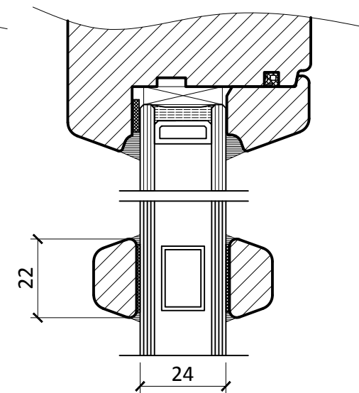
Splayed Profile 1
