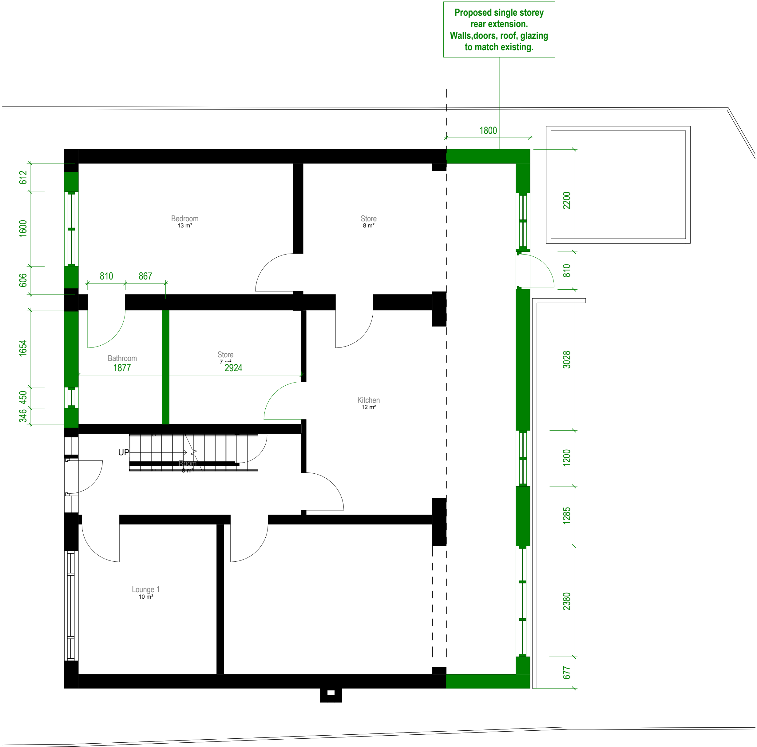
2 Level 0 Proposed 1 : 50
