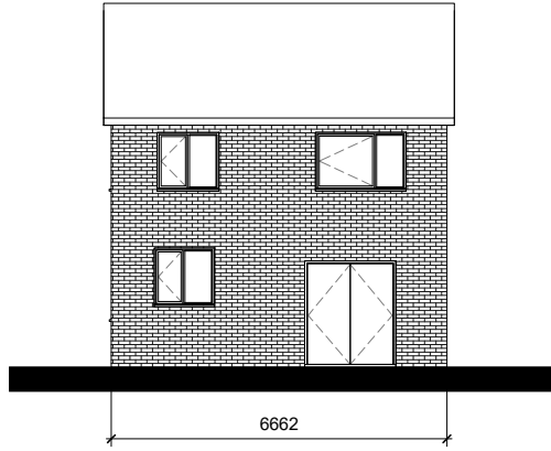
Existing East Elevation 1 : 100
