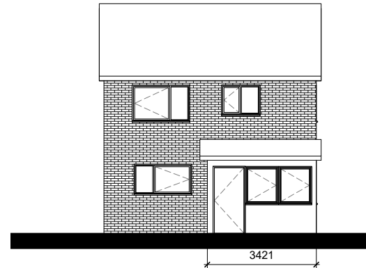
Existing West Elevation 1 : 100
