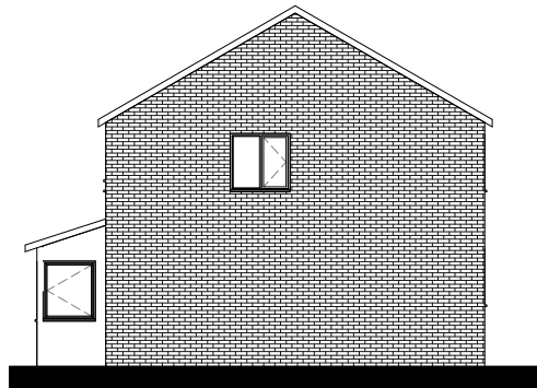
Existing South Elevation 1 : 100
