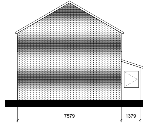
Existing North Elevation 1 : 100
