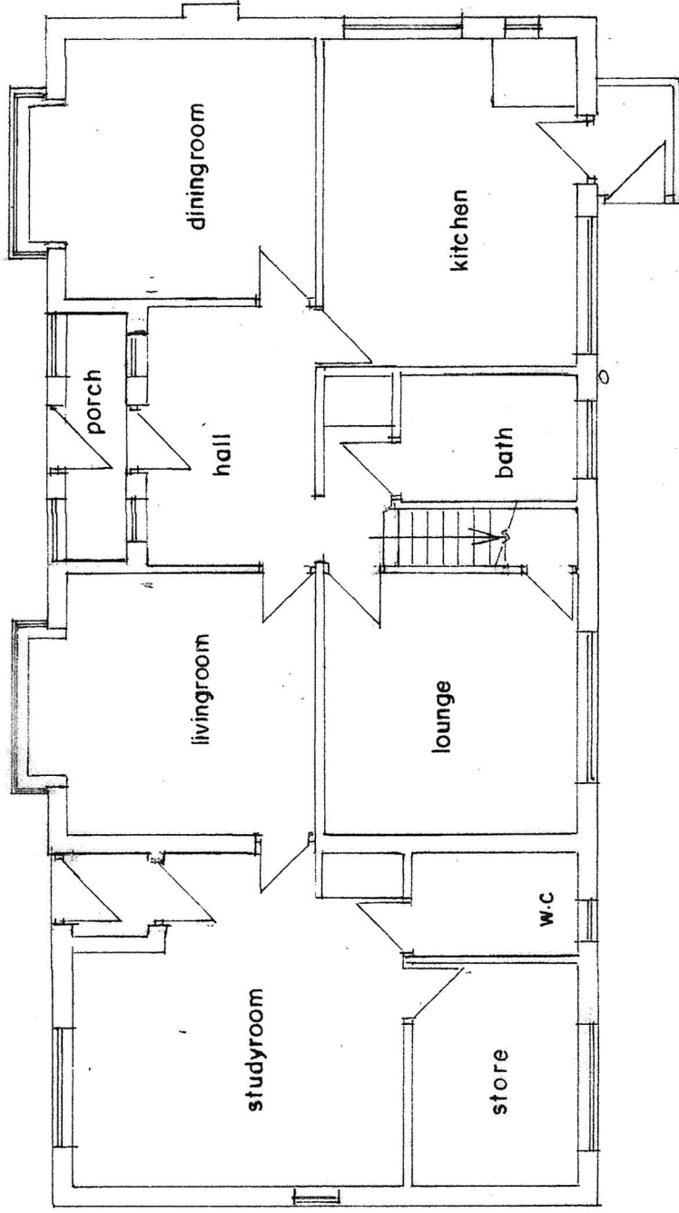
GROUND FLOOR PLAN (EXISTING)
