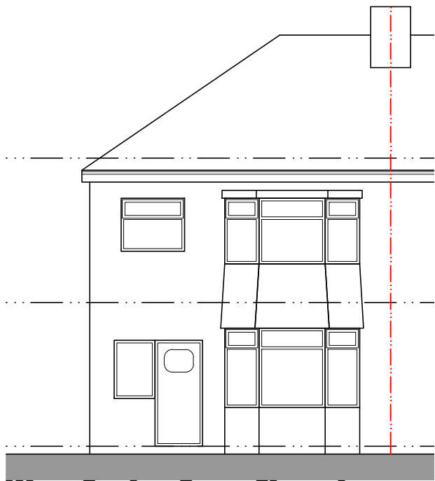
West Facing Front Elevation
