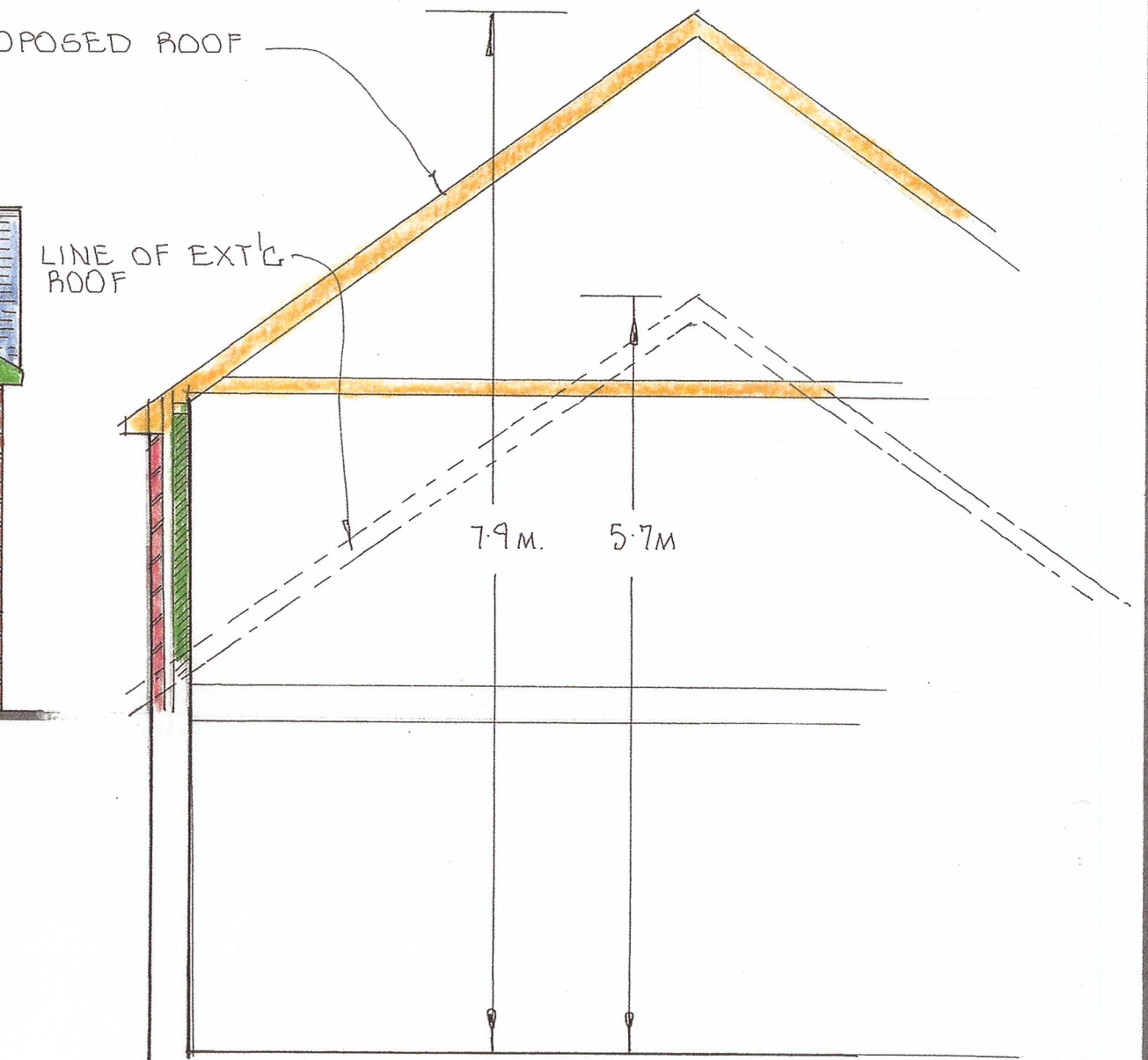
CROSS SECTION
