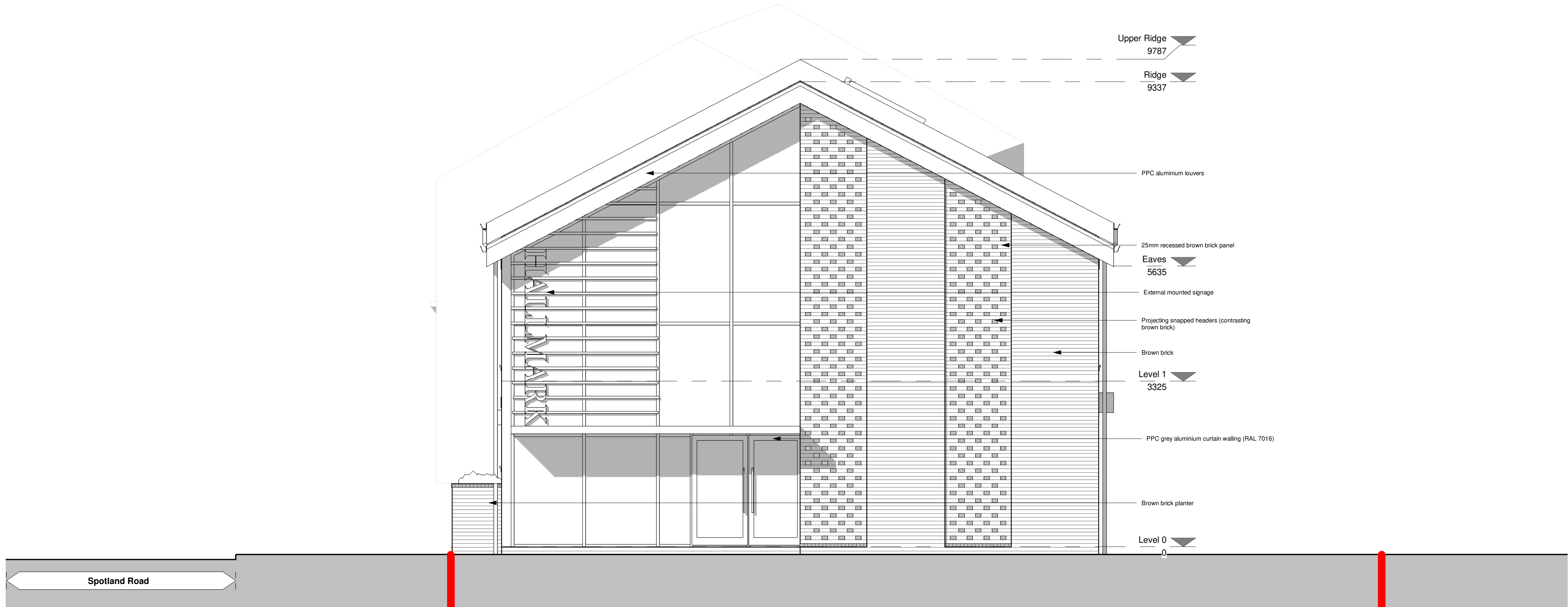
2 | Proposed West Elevation 1 : 50
