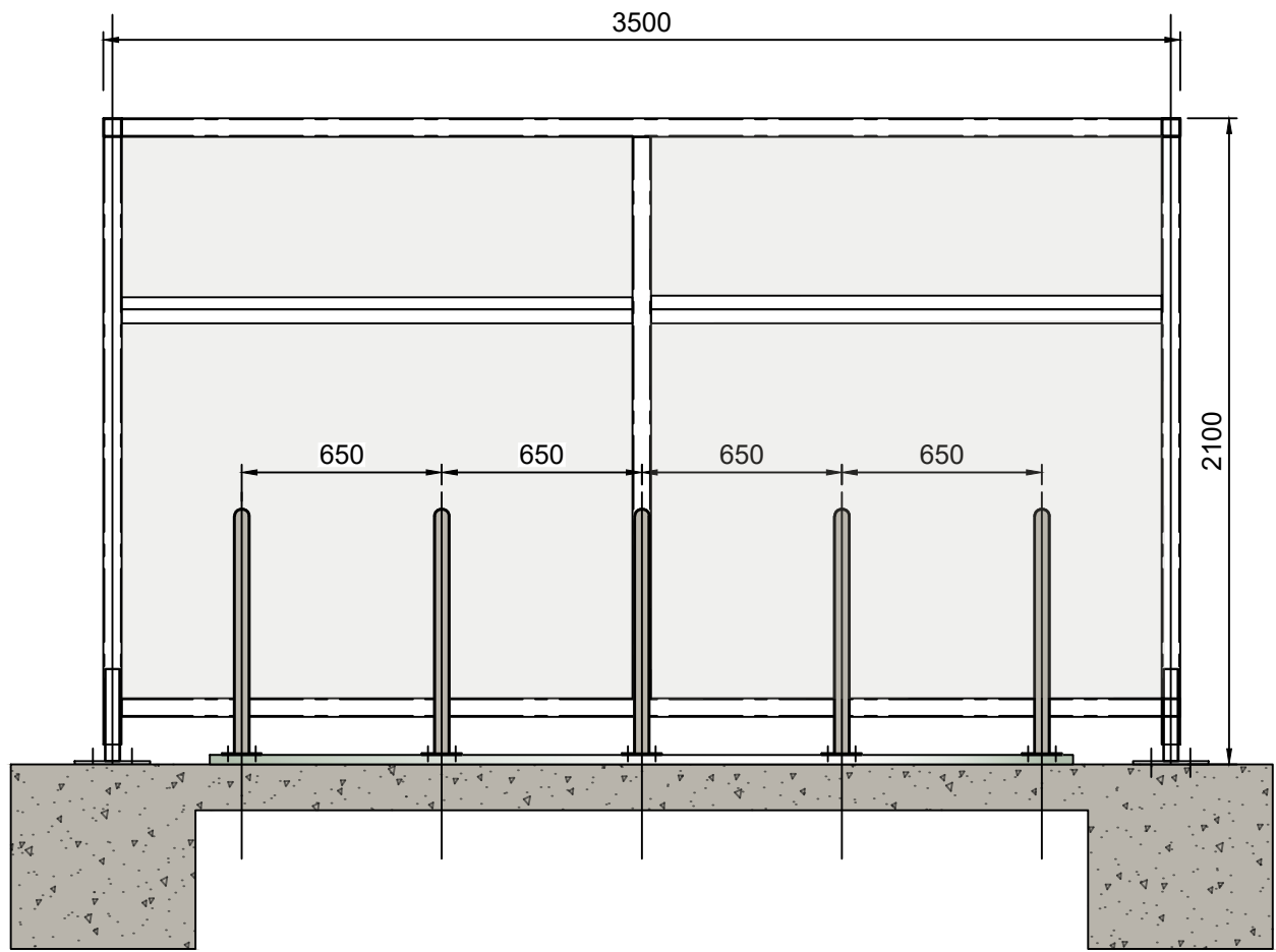
Proposed Cycle Shelter Elevations Scale 1:25 @ A1
