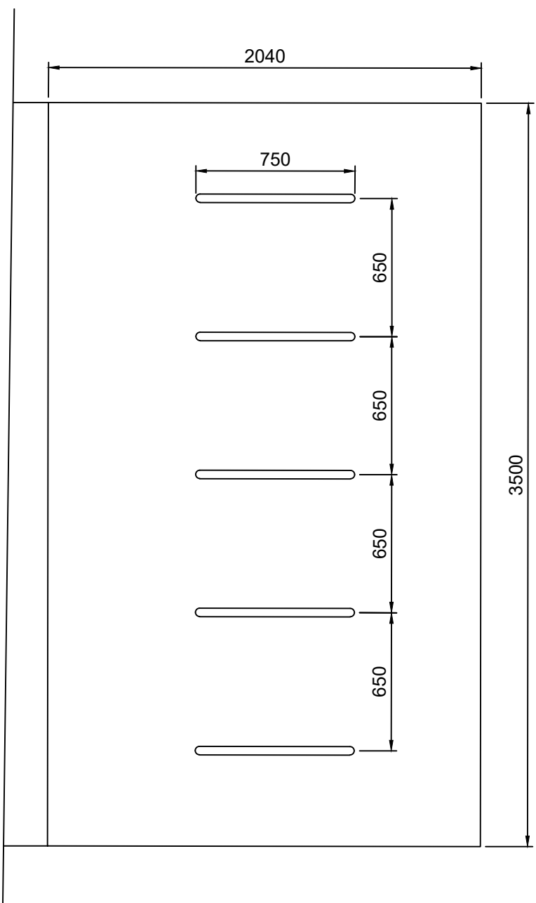
Proposed Cycle Shelter Plan Scale 1:25 @ A1
