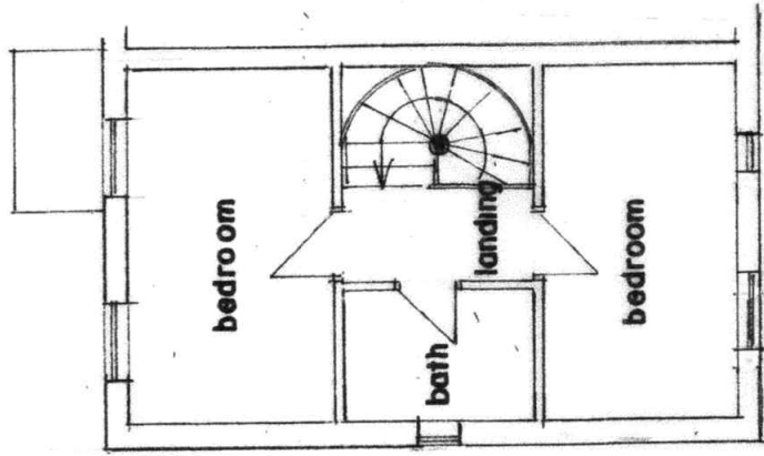
F.F. PLAN (EXISTING)
