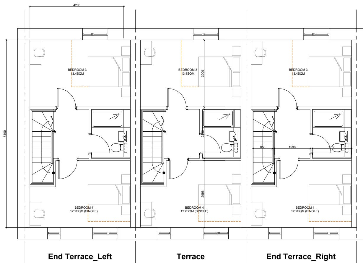
4 BED 6P - SECOND FLOOR Floor Area: 37.80 sq.m.
