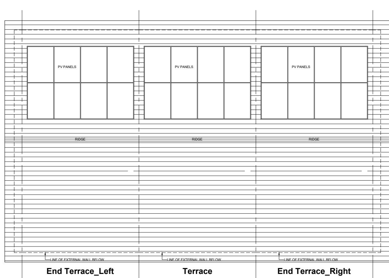
4 BED 6P - ROOF
