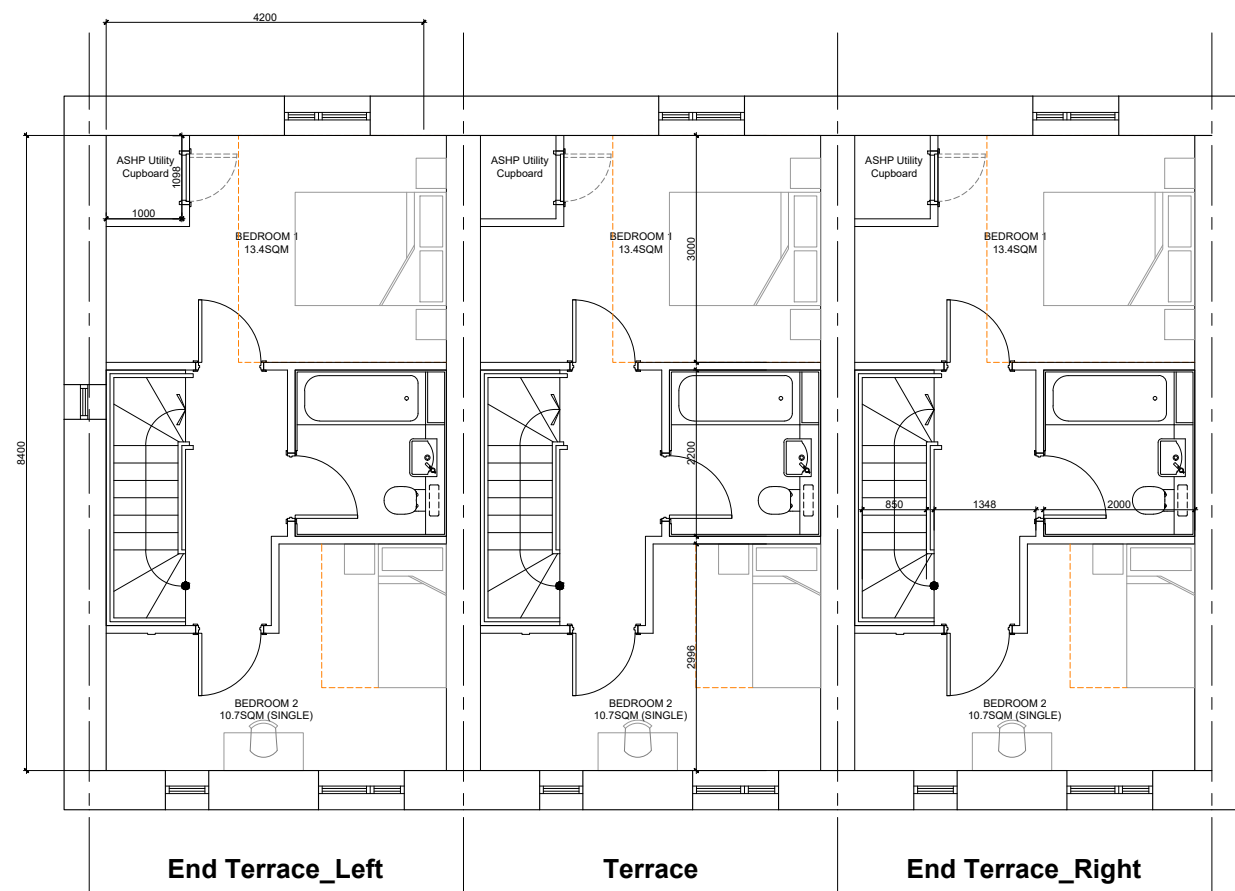
4 BED 6P - FIRST FLOOR Floor Area: 37.80 sq.m. Total Area: 113.40 sq.m (112 sq.m)
