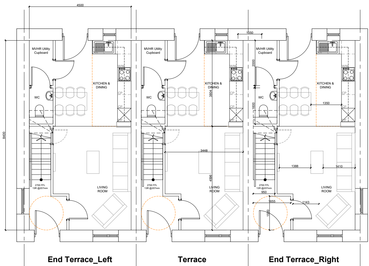
4 BED 6P - GROUND FLOOR Floor Area: 37.80 sq.m.
