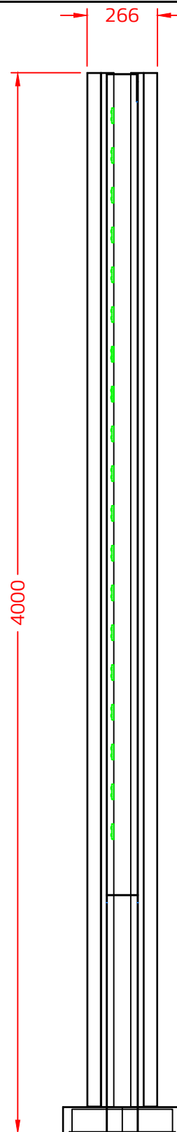
SIDE VIEW
