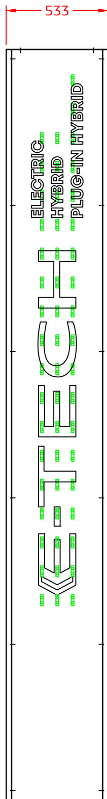
FACE VIEW
