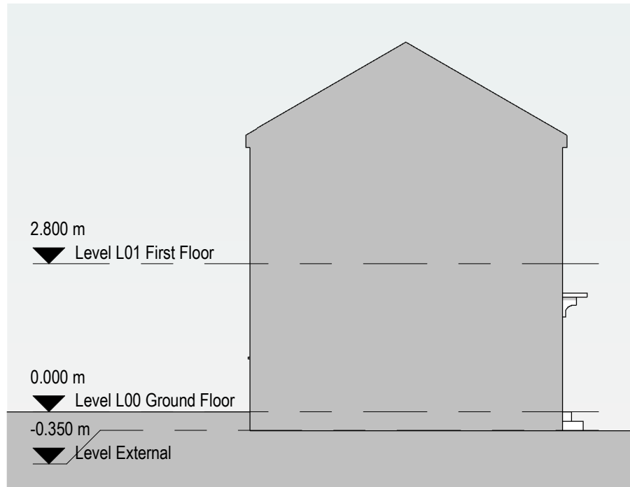
4 Existing East Elevation 1 : 100
