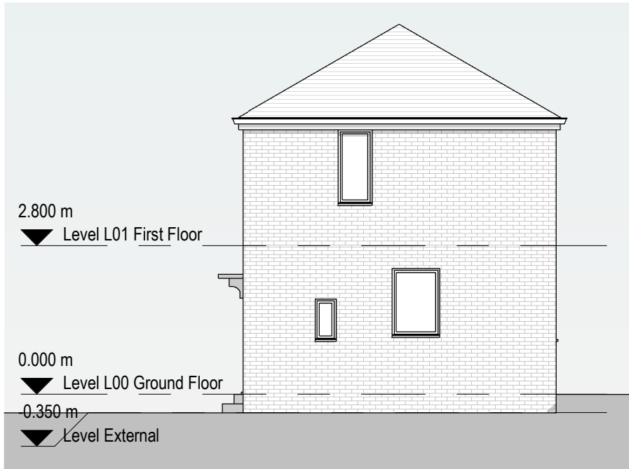
2 Existing West Elevation 1 : 100
