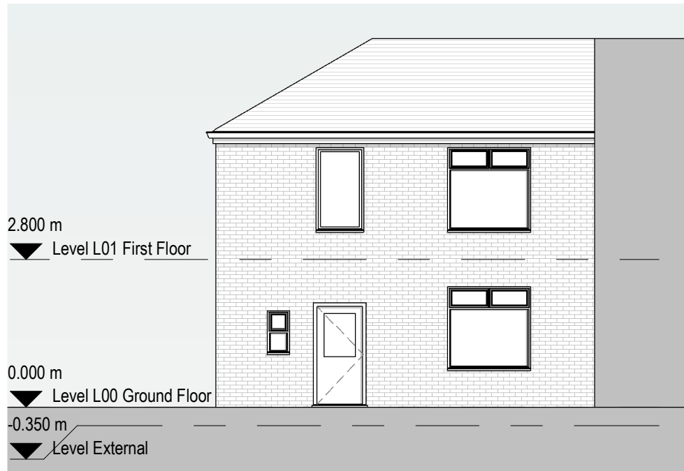
3 Existing South Elevation 1 : 100
