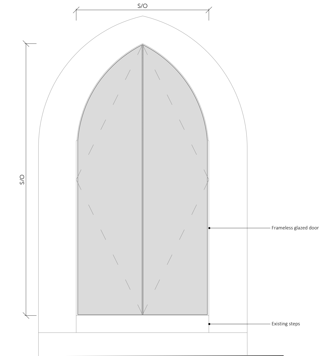
1 Glazed Double Leaf, External
