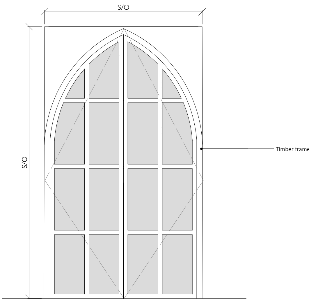
2 Glazed Double Leaf, Internal
