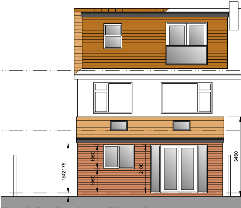
North Facing Rear Elevation
