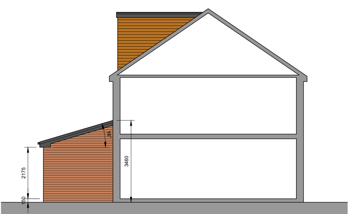
West Facing Side Elevational Section
