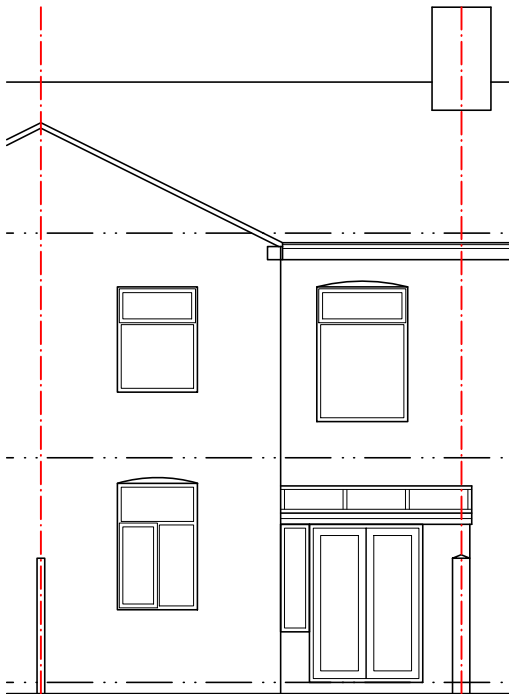
North Facing Rear Elevation
