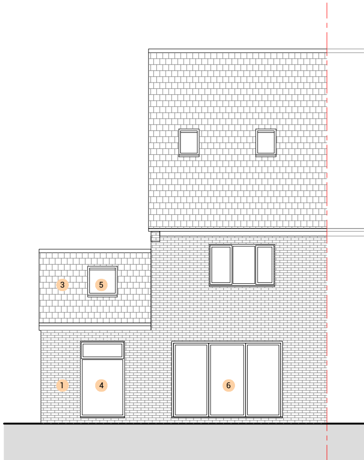
PROPOSED REAR ELEVATION 1:100 @ A3
