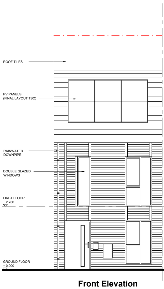
Front Elevation
