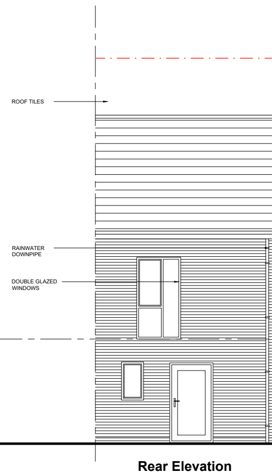
Rear Elevation
