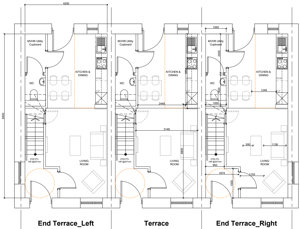
2 BED 3P - GROUND FLOOR Floor Area: 35.27 sq.m.
