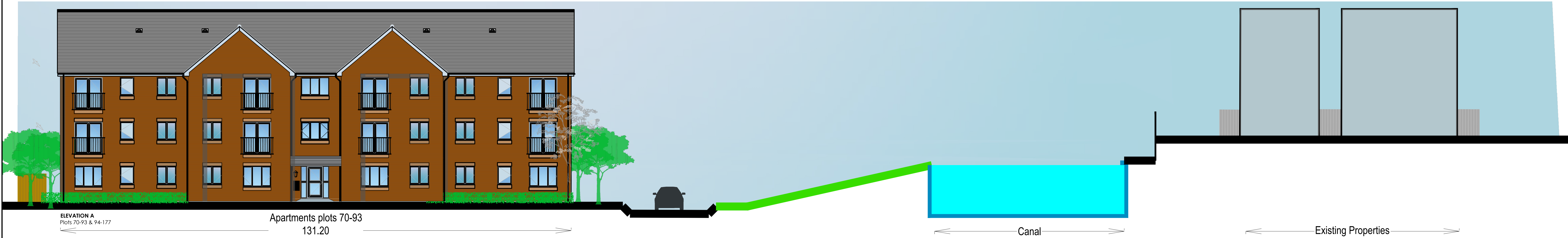
SECTION E-E
