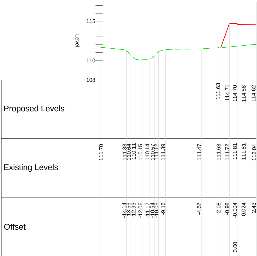
SECTION K-K
