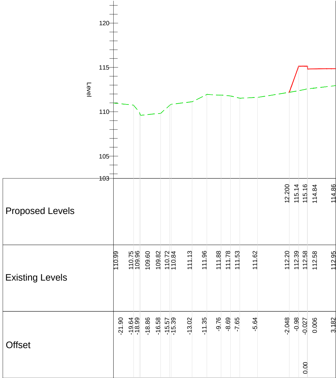
SECTION J-J
