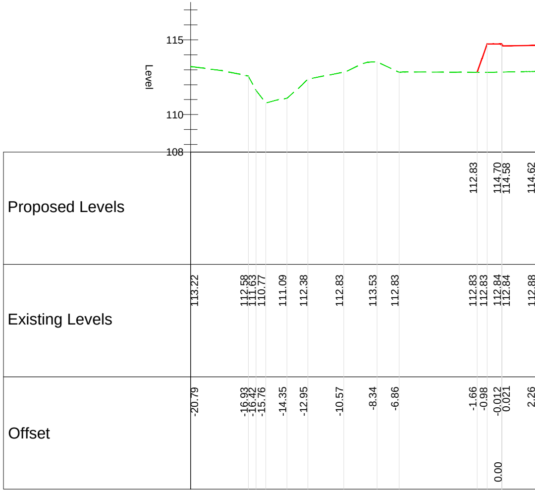
SECTION M-M
