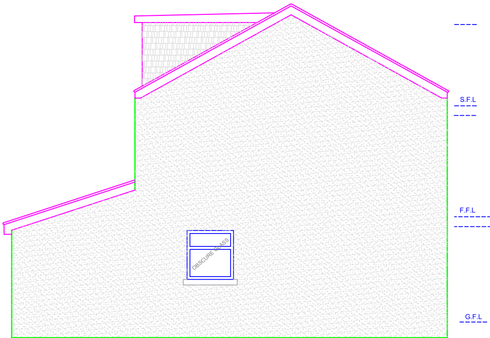
PROPOSED REAR ELEVATION (EAST)
