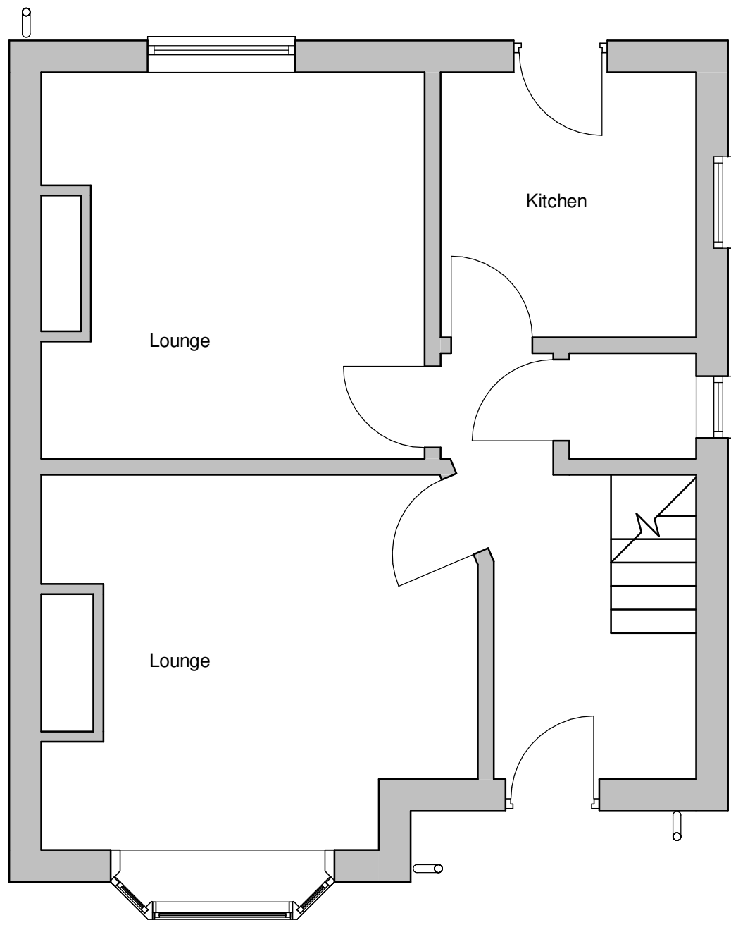
Existing Ground Floor 1 : 50
