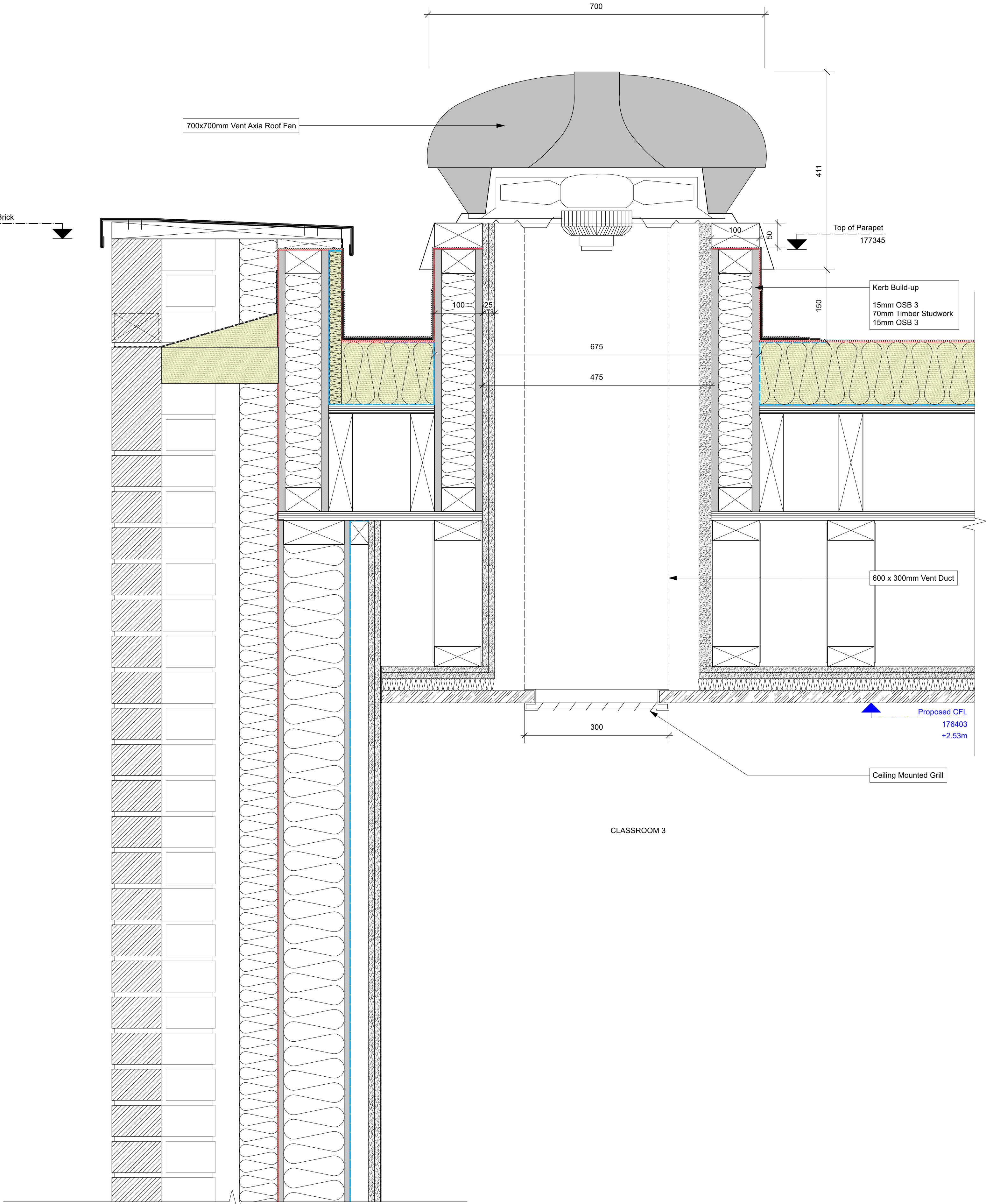
1 Roof Cowl Section Detail Scale: 1:5
