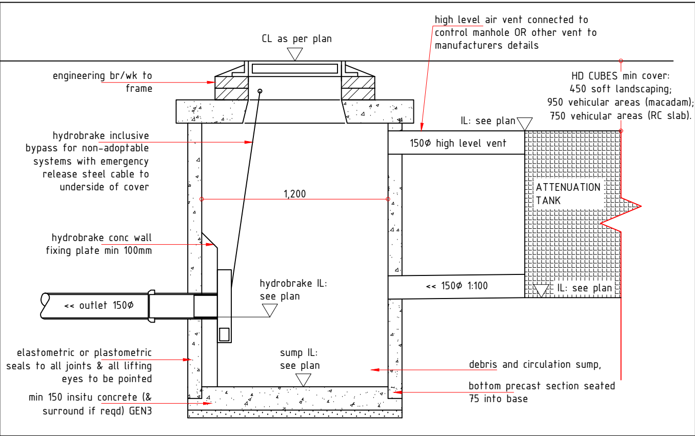
typical control manhole detail detail (1:10)
