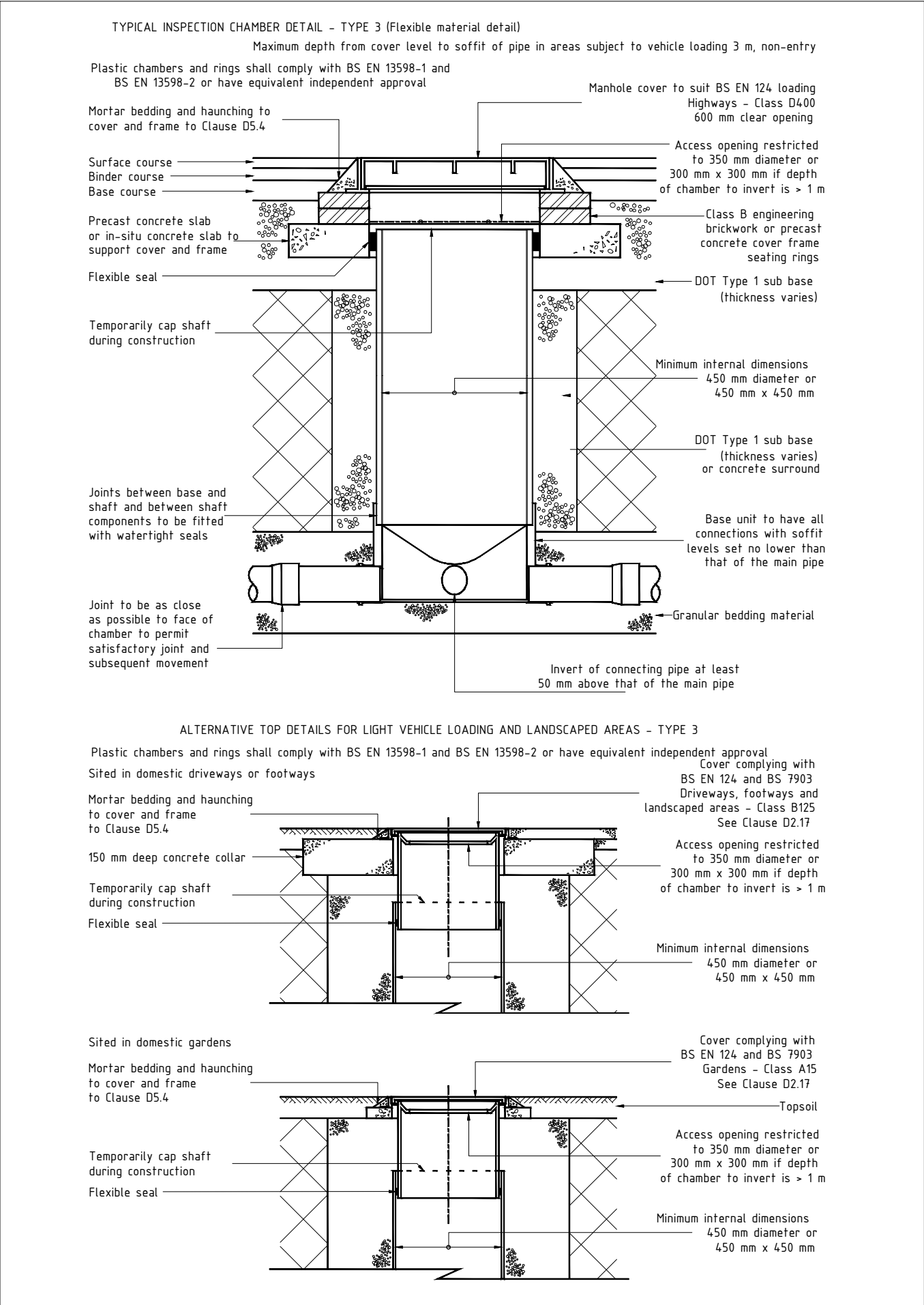
typical inspection chamber detail (1:10)
