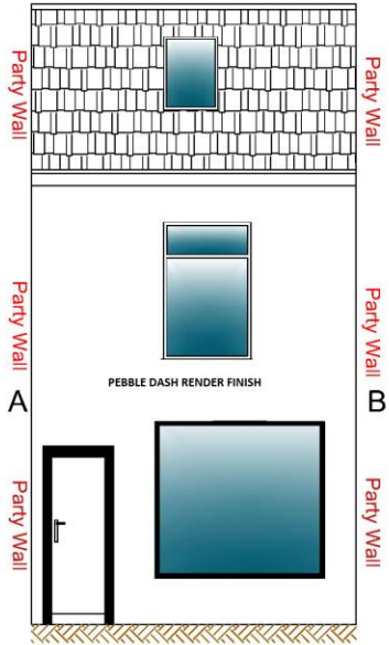
EXISTING FRONT ELEVATION 1:50 @ A1
