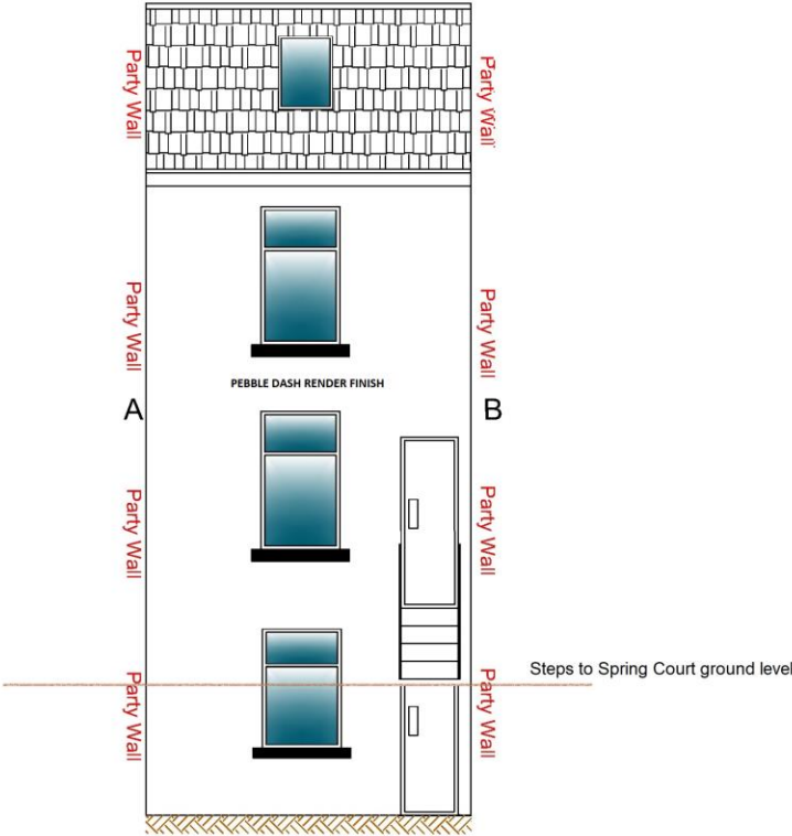
EXISTING REAR ELEVATION 1:50 @ A1
