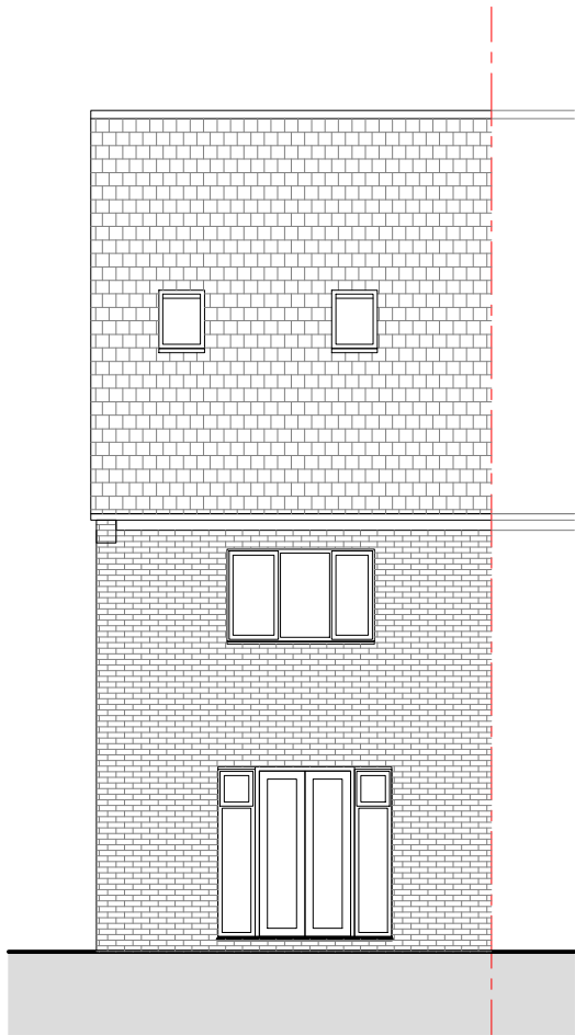
EXISTING REAR ELEVATION 1:100 @ A3
