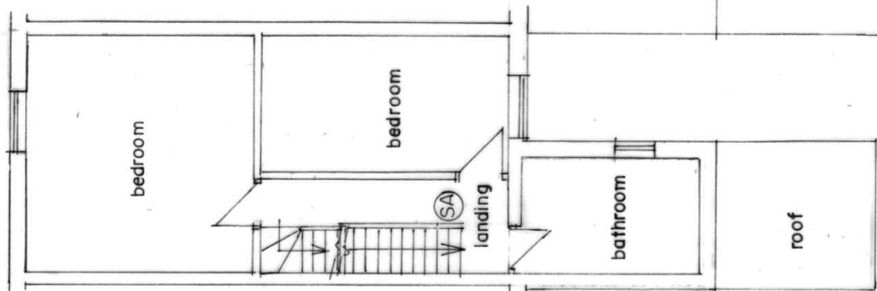
SECOND FLOOR PLAN (PROPOSED)
