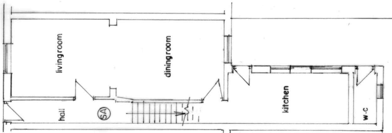
GROUND FLOOR PLAN (PROPOSED)
